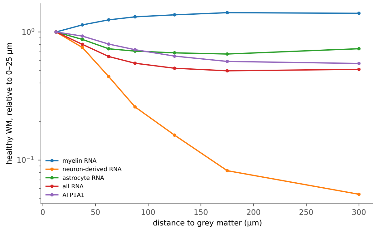
healthy white matter: gradients away from grey matter
