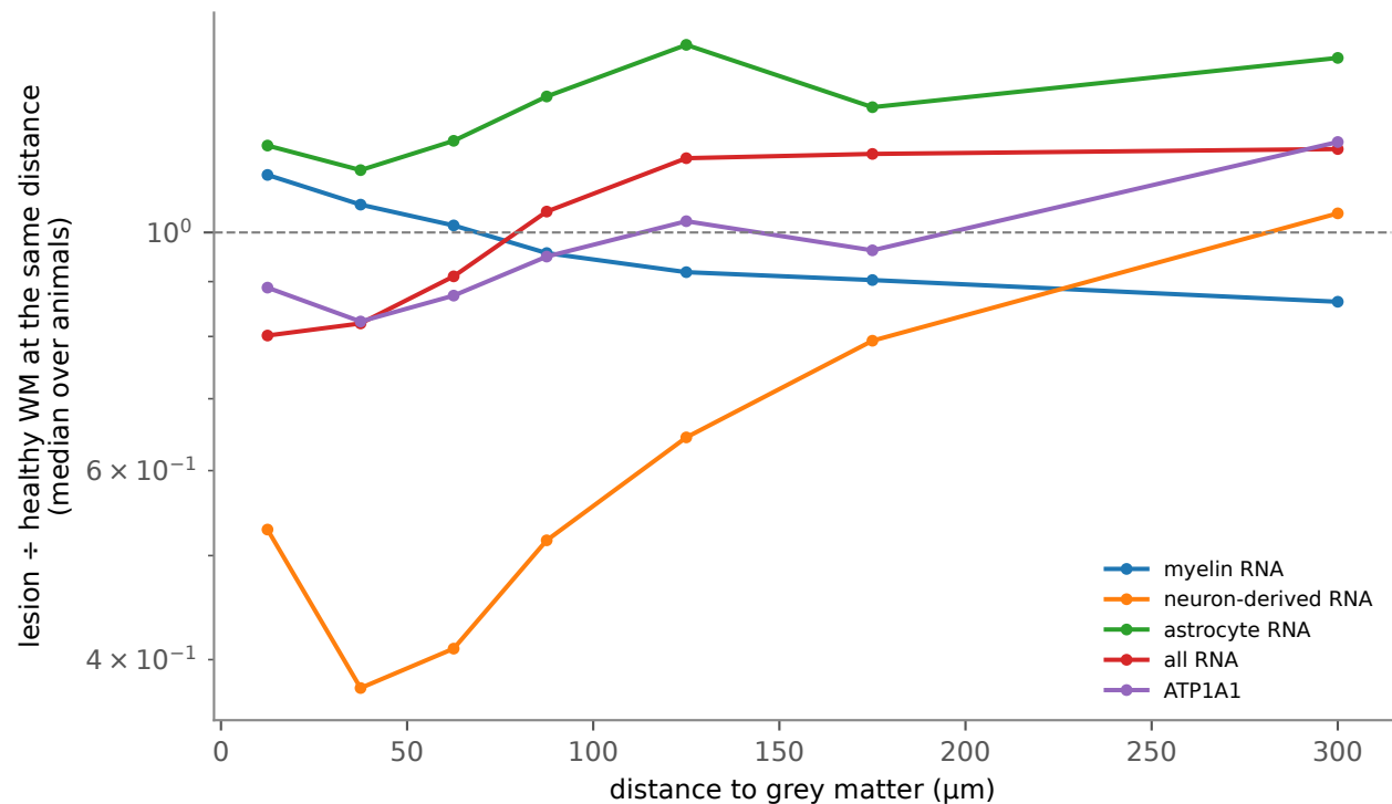
distance-matched lesion effect
