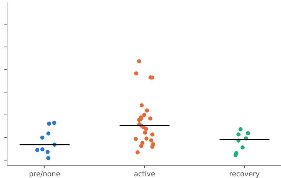
runs 1-3: \rho(\text{protein, RNA}) = 0.54
