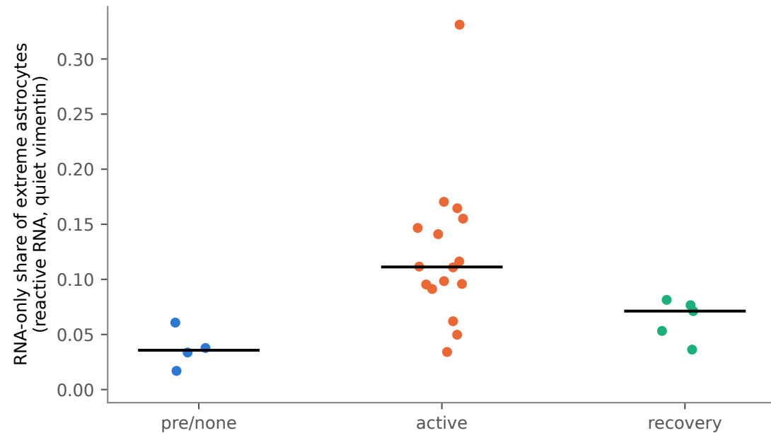
runs 5/6: \rho(\text{protein, RNA}) = 0.48
