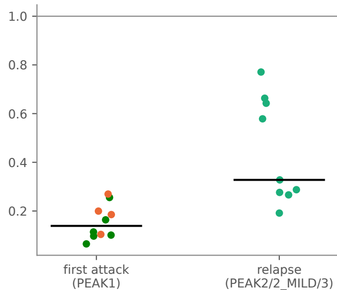
adjacency: observed \div permutation
