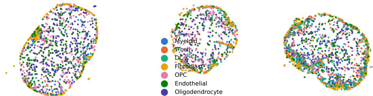
transcriptome annotation (7 most frequent types)
