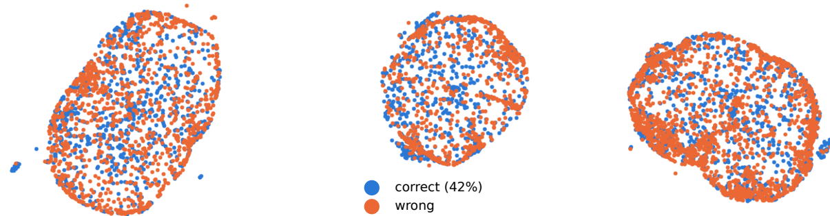
image-only cell-type prediction, run6_S5-B2_0085405 (CV, held-out animals)
