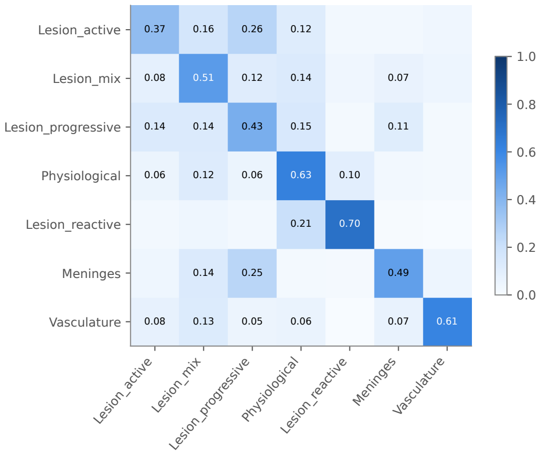
lesion state from images only
