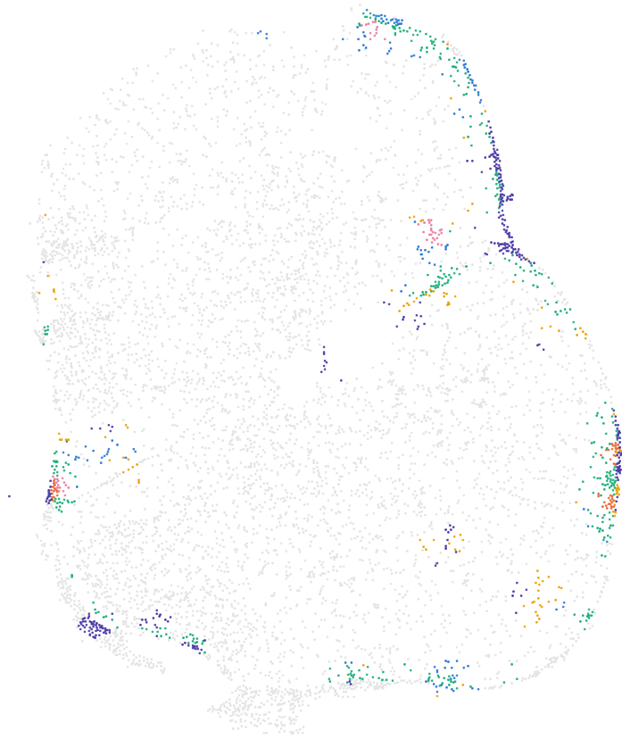
lesion states
