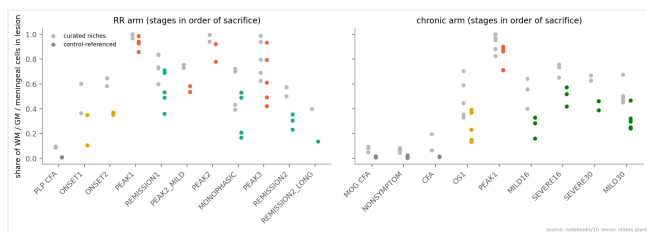
Figure 2a · Lesion share per animal: curated labels (grey) vs control-referenced (coloured).
