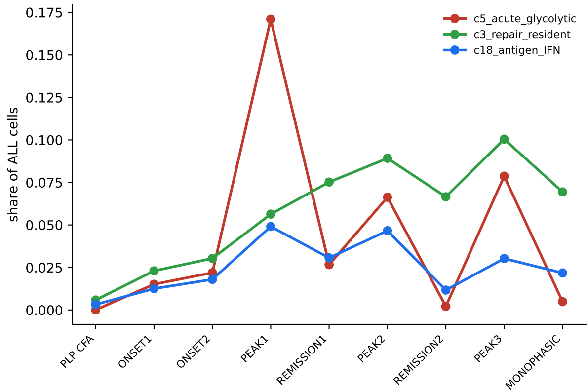
Myeloid state as % of all cells
