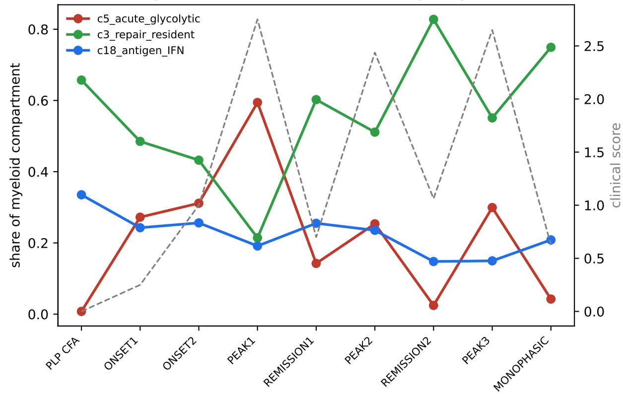
Myeloid state share across the relapse cycle
