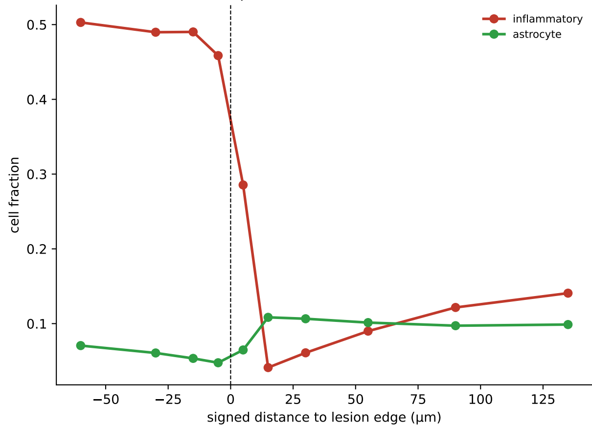
Composition vs radial distance
