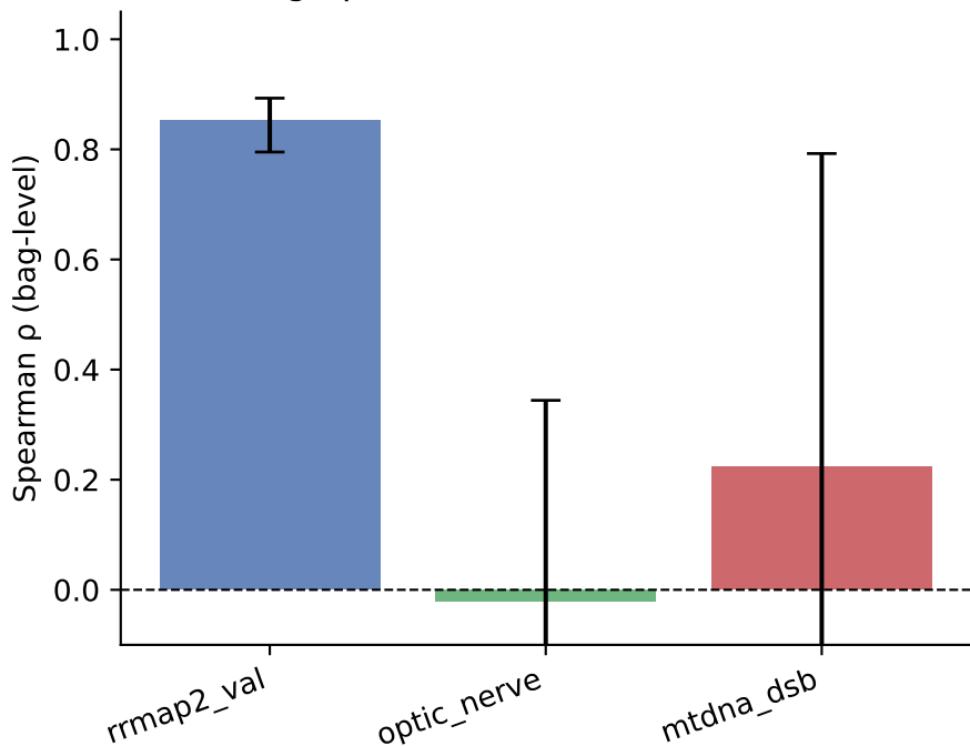
Disease stage prediction: within-domain vs. transfer
