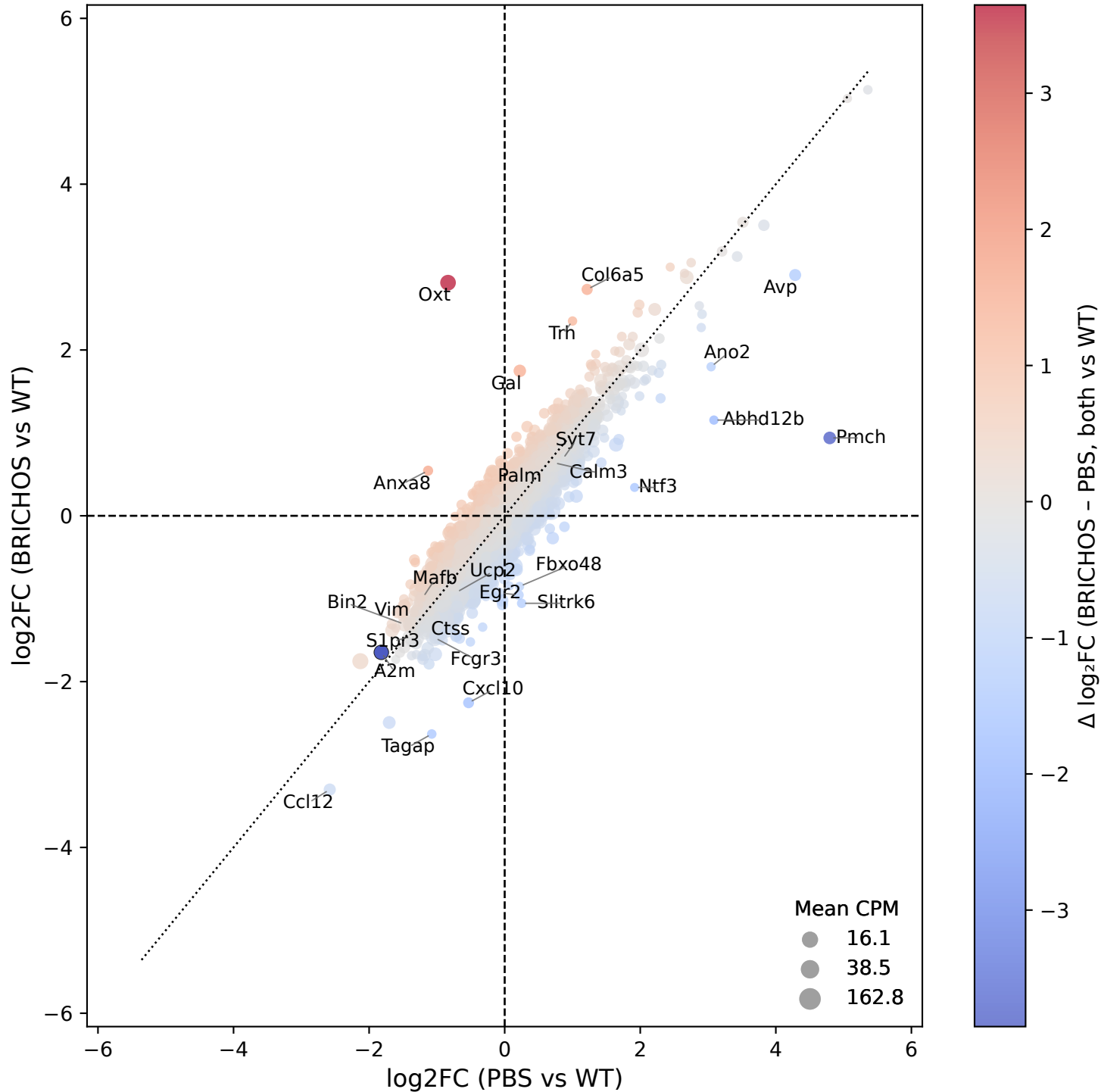
Corpus callosum: PBS vs WT vs BRICHOS vs WT (LFC prioritized; size ~ expression, min_cpm=3)
