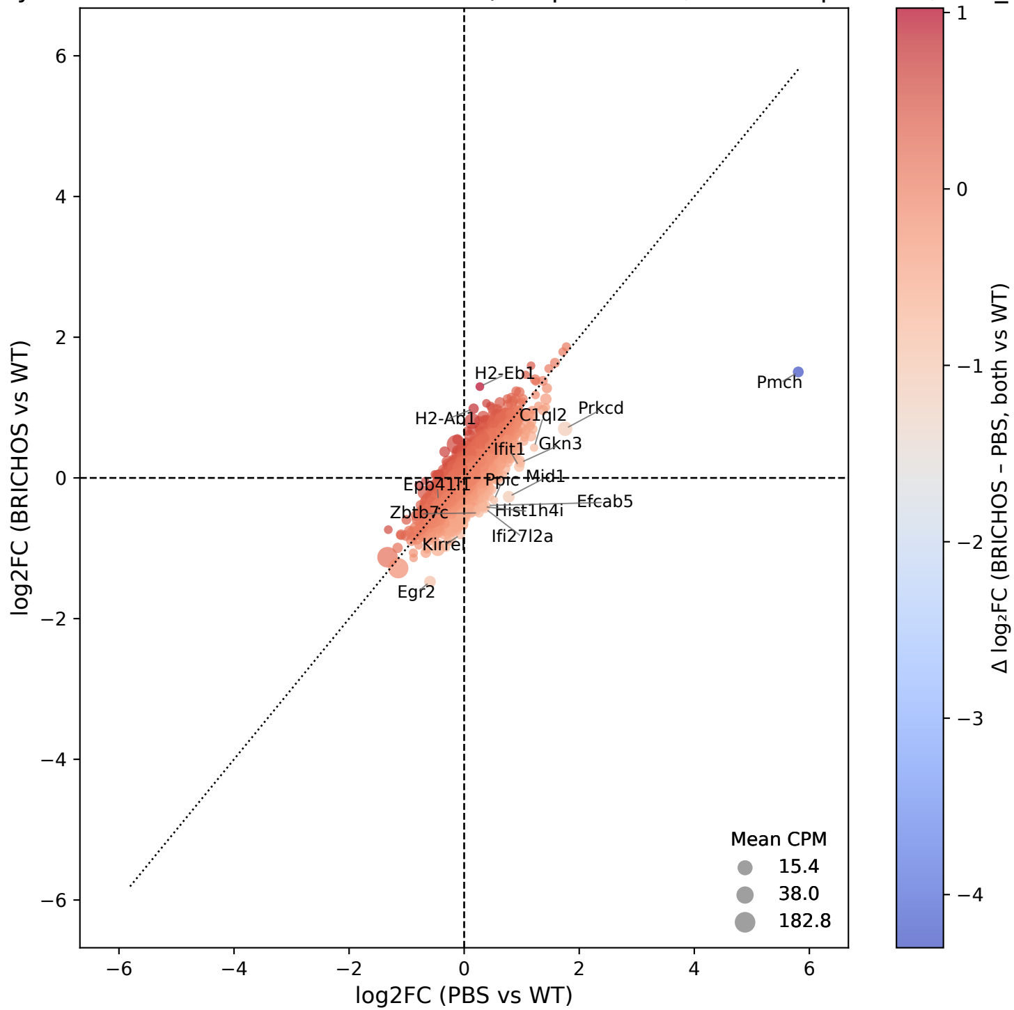
Infragranular layers: PBS vs WT vs BRICHOS vs WT (LFC prioritized; size ~ expression, min_cpm=3)
