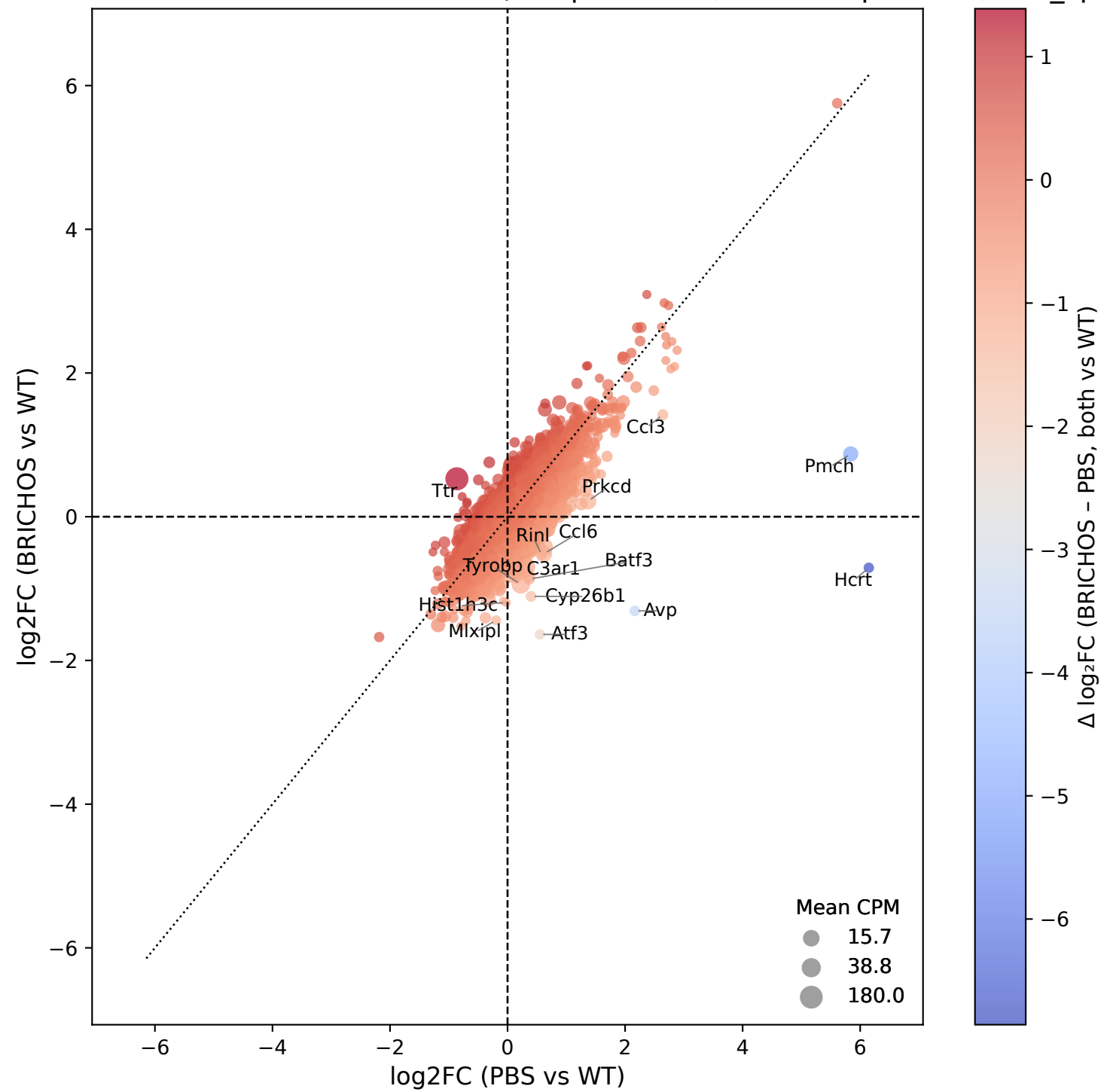
Olfactory areas: PBS vs WT vs BRICHOS vs WT (LFC prioritized; size ~ expression, min_cpm=3)
