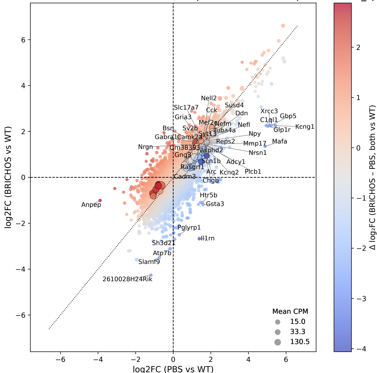
Ventricular area: PBS vs WT vs BRICHOS vs WT (LFC prioritized; size ~ expression, min_cpm=3)
