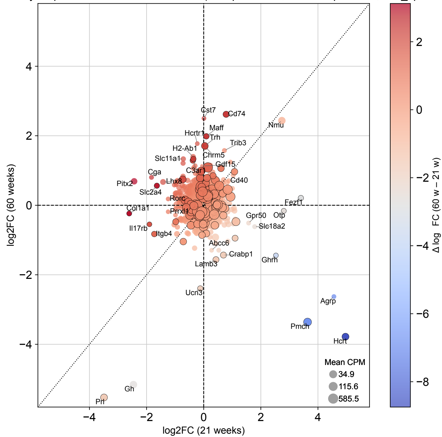
Oligodendrocytes precursor cells: 21 w vs 60 w (LFC prioritized; size ~ expression, min_cpm=3)
