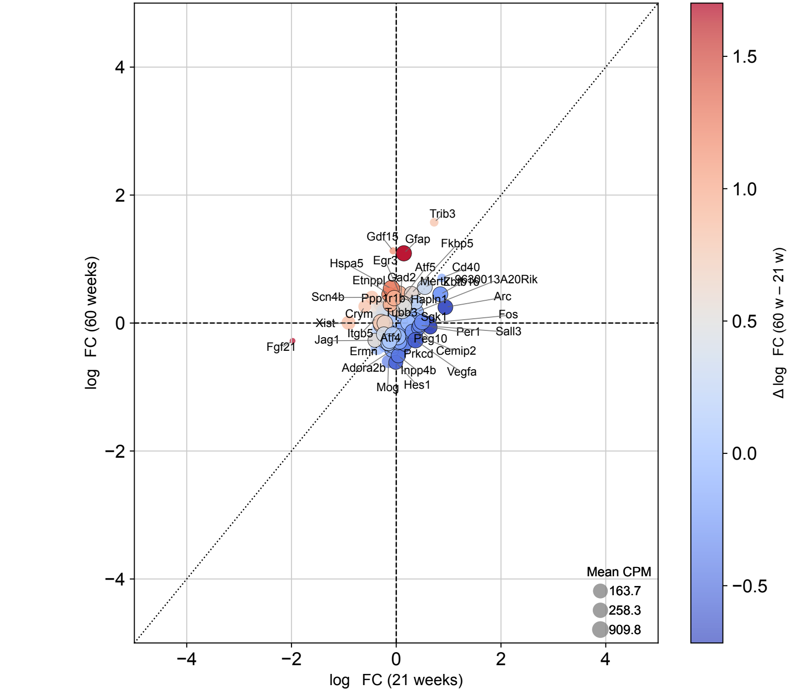
Oligodendrocytes precursor cells: 21 w vs 60 w (LFC prioritized; size ~ expression, min_cpm=100)
