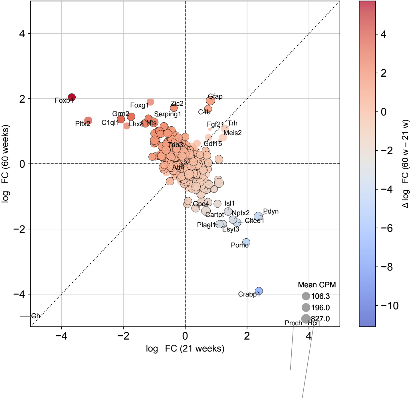
Neurons: 21 w vs 60 w (LFC prioritized; size ~ expression, min_cpm=50)
