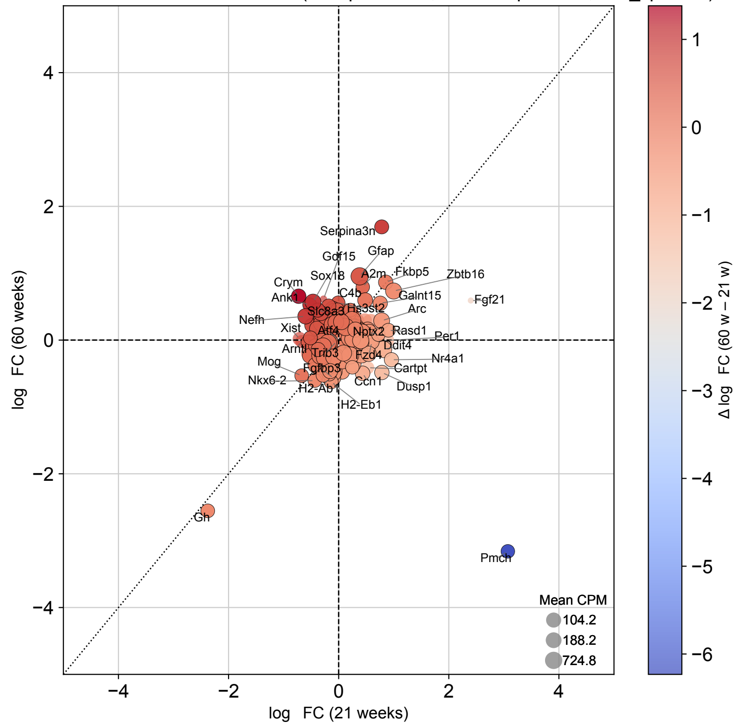
Vascular endothelial cells: 21 w vs 60 w (LFC prioritized; size ~ expression, min_cpm=50)
