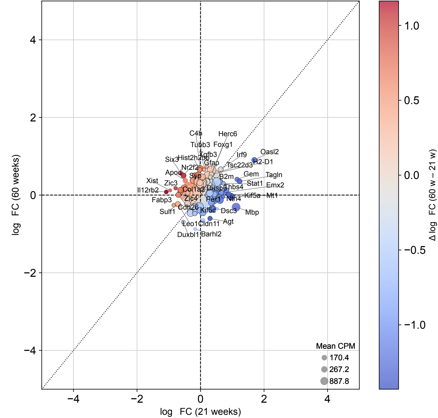
Ependymal cells: 21 w vs 60 w (LFC prioritized; size ~ expression, min_cpm=100)
