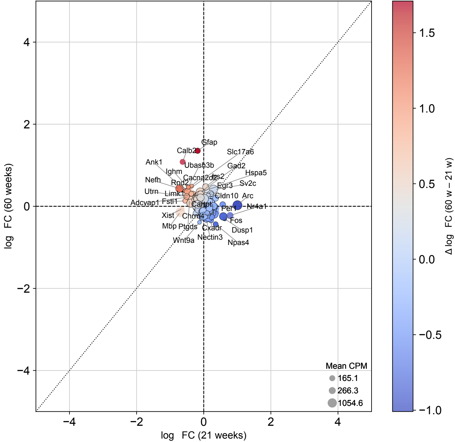
Excitatory neurons: 21 w vs 60 w (LFC prioritized; size ~ expression, min_cpm=100)
