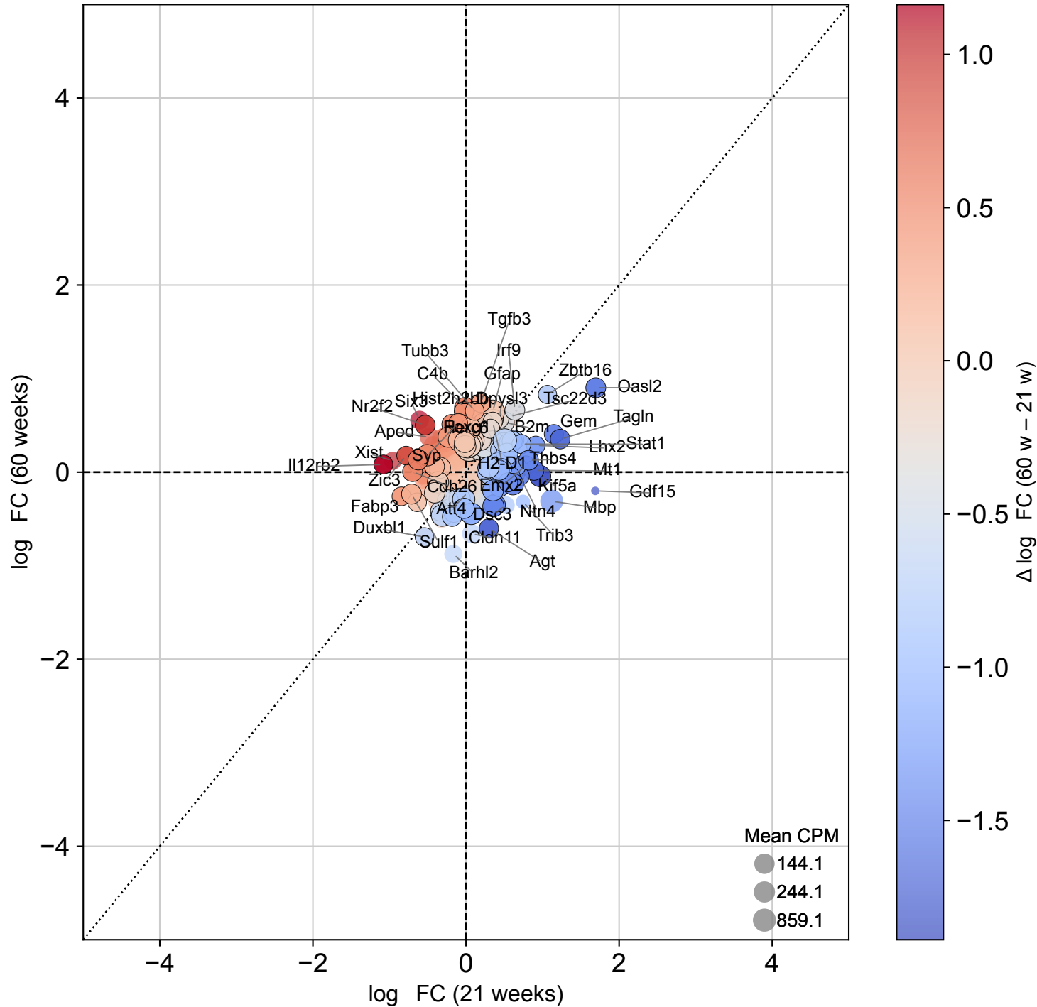
Ependymal cells: 21 w vs 60 w (LFC prioritized; size ~ expression, min_cpm=80)
