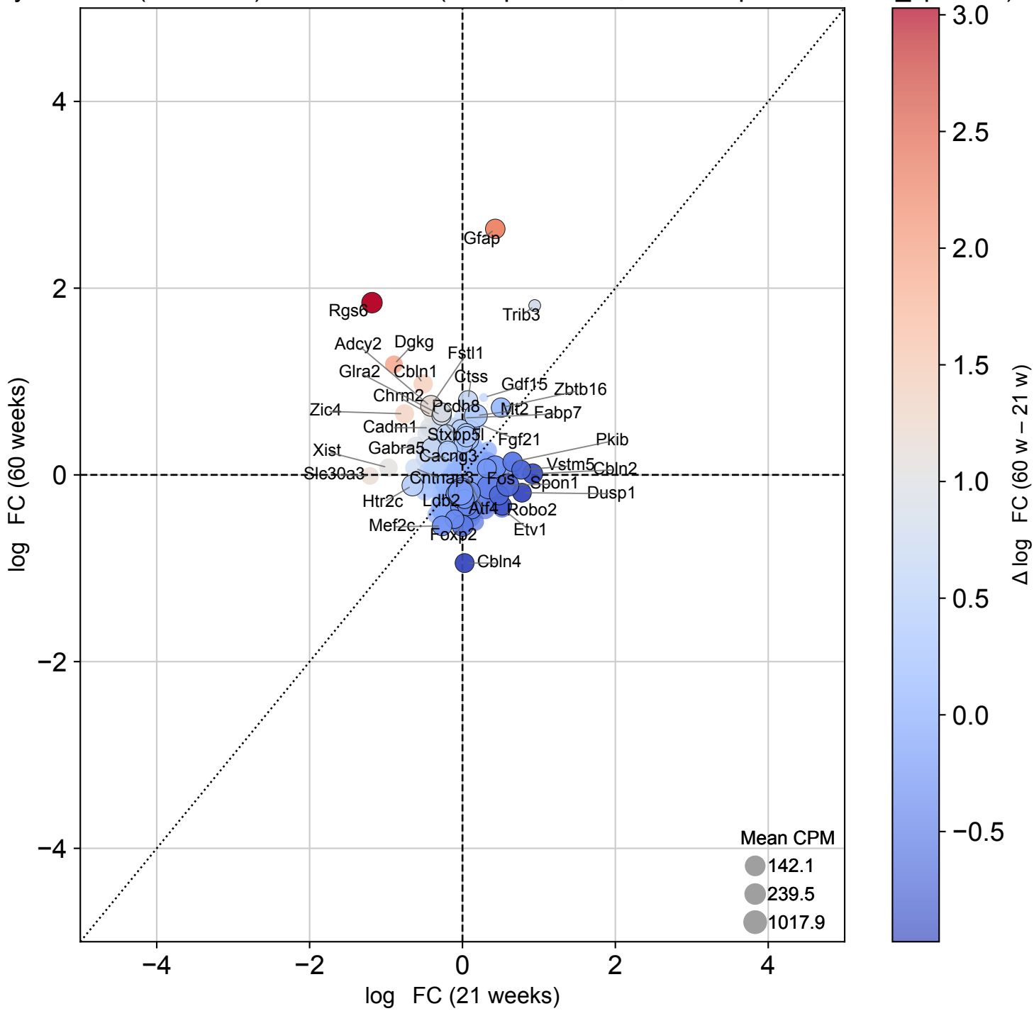
Excitatory neurons (thalamus): 21 w vs 60 w (LFC prioritized; size ~ expression, min_cpm=80)
