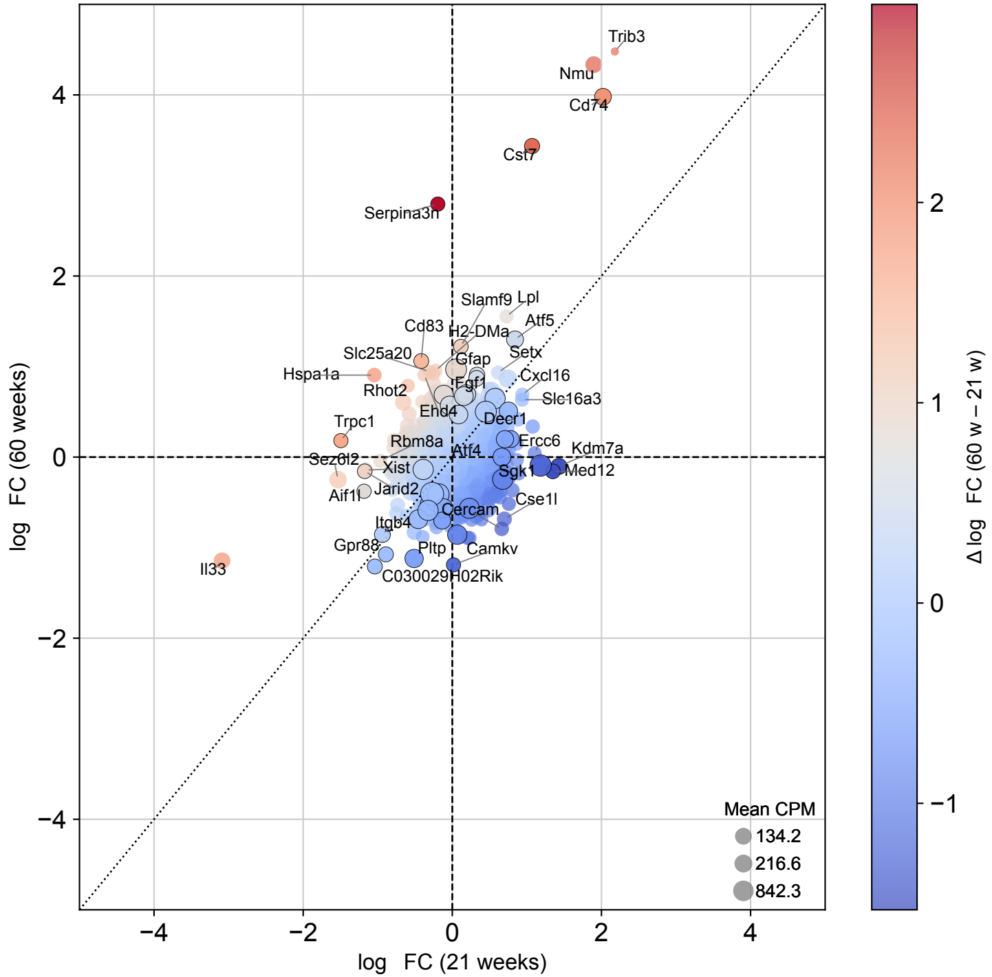
Mature oligodendrocytes (mic): 21 w vs 60 w (LFC prioritized; size ~ expression, min_cpm=80)
