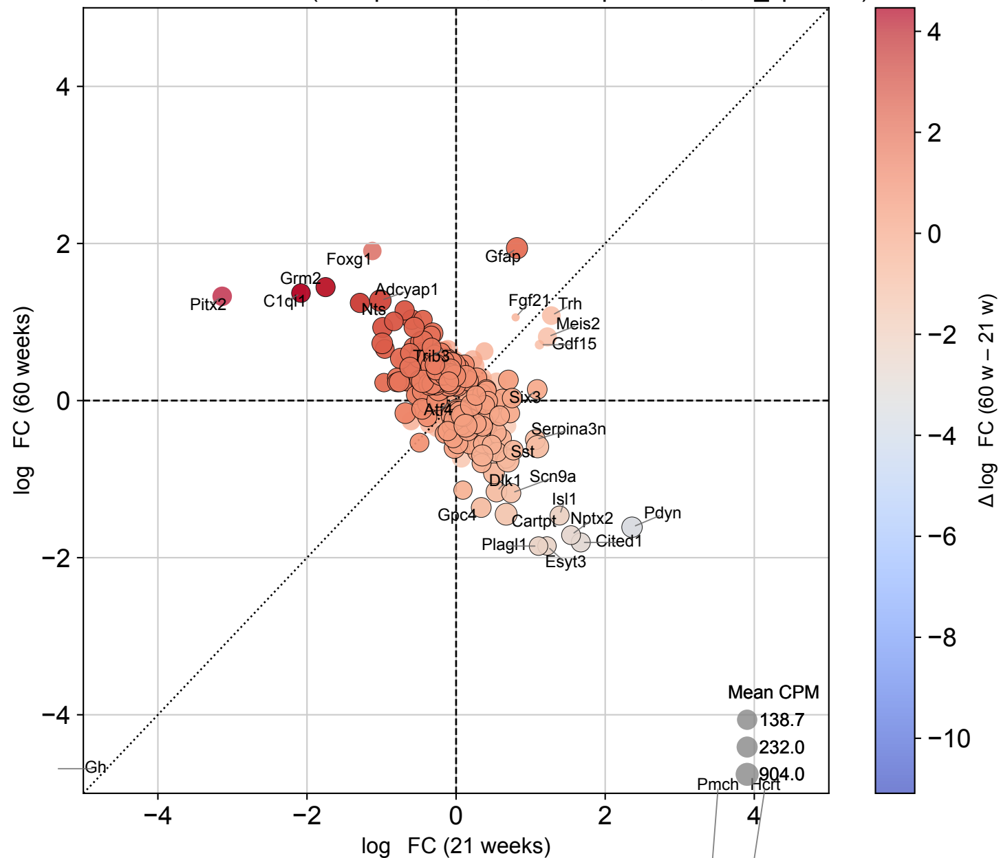
Neurons: 21 w vs 60 w (LFC prioritized; size ~ expression, min_cpm=80)
