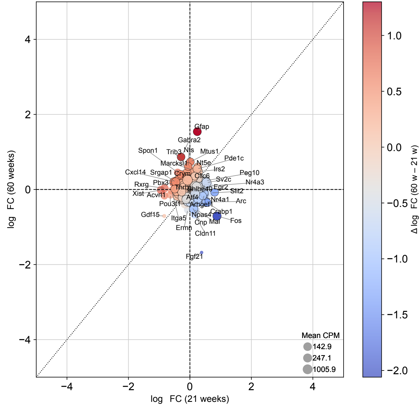
Striatal neurons: 21 w vs 60 w (LFC prioritized; size ~ expression, min_cpm=80)
