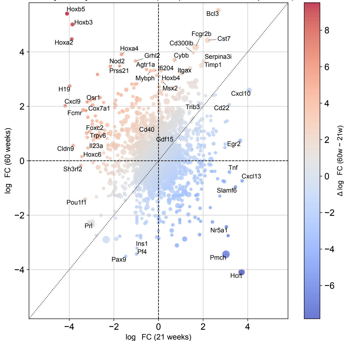
Olfactory astrocytes: 21w vs 60w (LFC-prioritized; size ~ expression)
