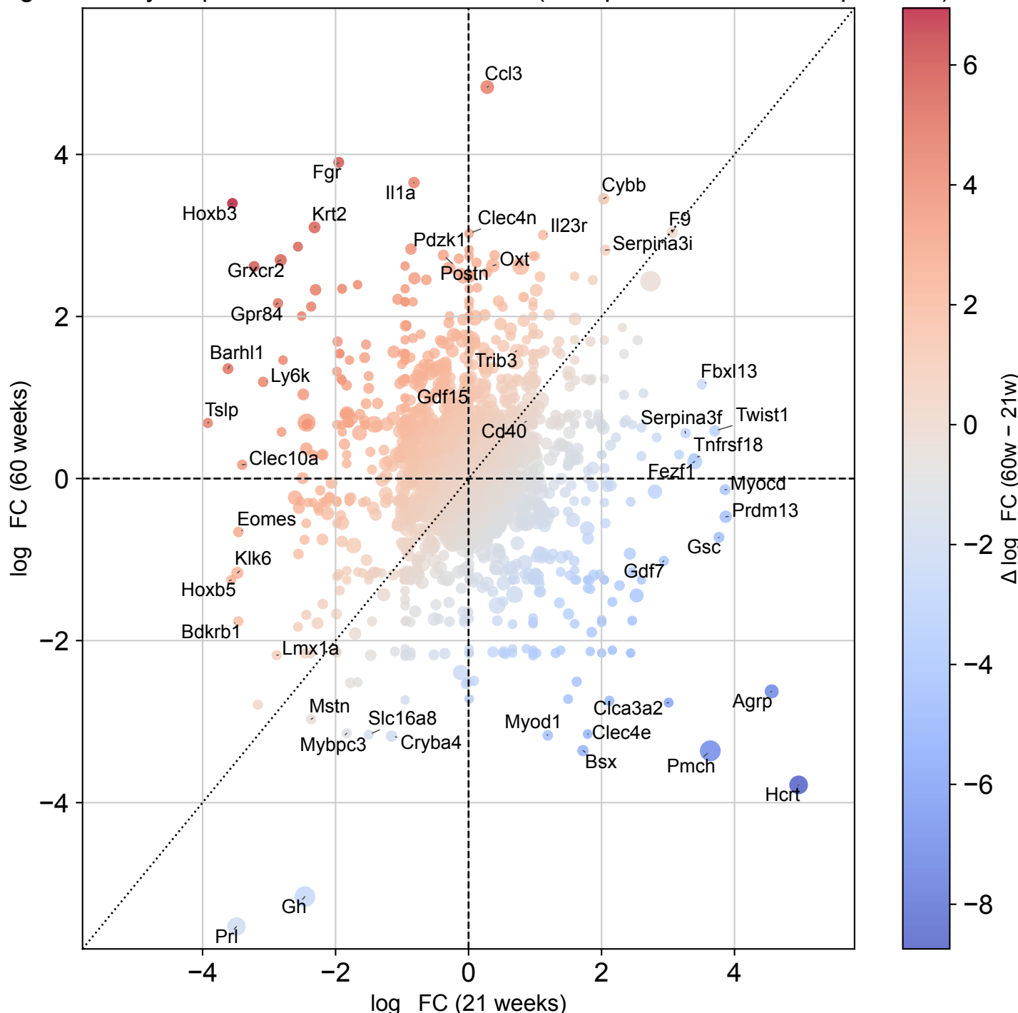
Oligodendrocytes precursor cells: 21w vs 60w (LFC-prioritized; size ~ expression)
