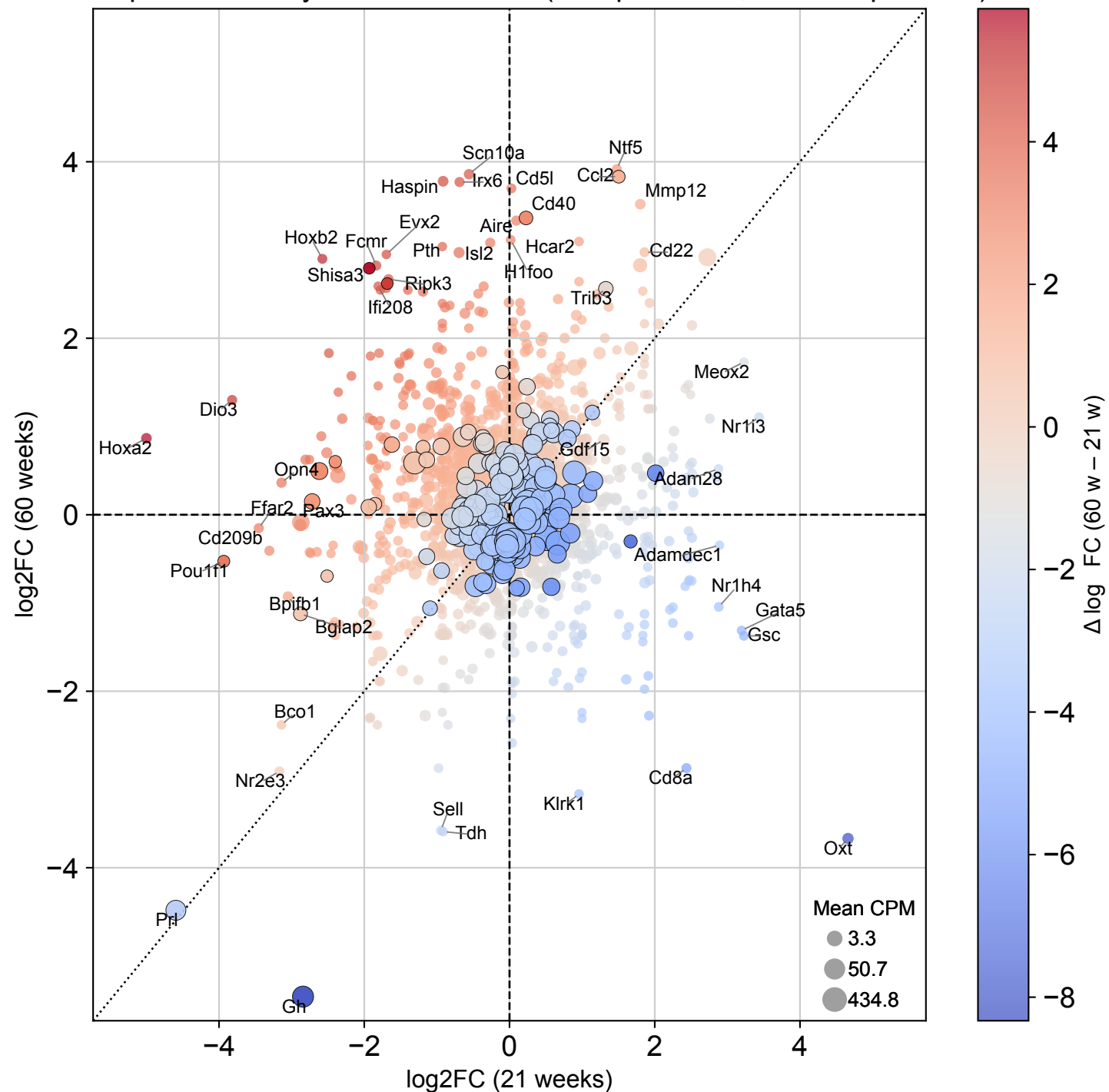
Telencephalon astrocytes: 21 w vs 60 w (LFC prioritized; size ~ expression)
