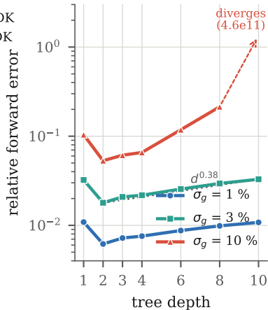
(b) error accumulation
