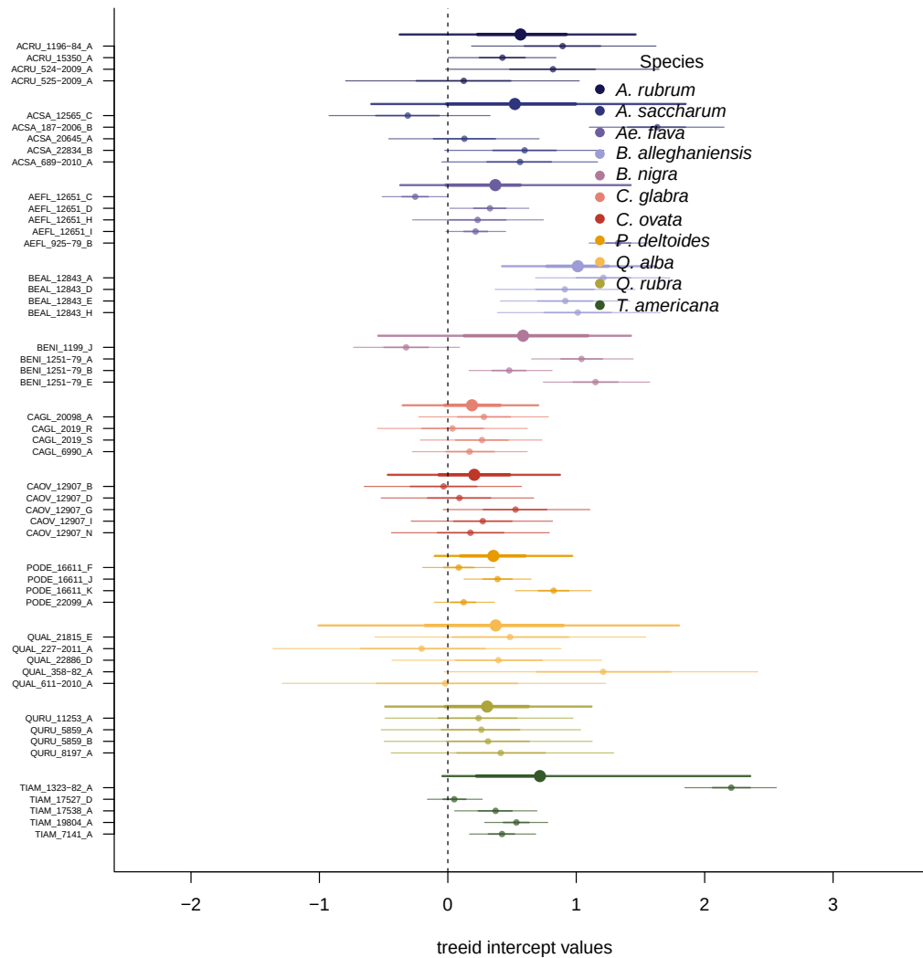
Figure S3: Intercept estimates for each group of the GDD model. The different tree id values represent the sum of the tree id, provenance, species and averaged year intercepts. The larger dots and lines represent aggregated average across these values. The dots are the mean of the posterior distribution and the thick and thin lines, the 50 and 90% UI.
