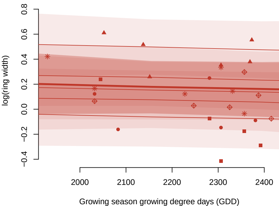
C. ovata
