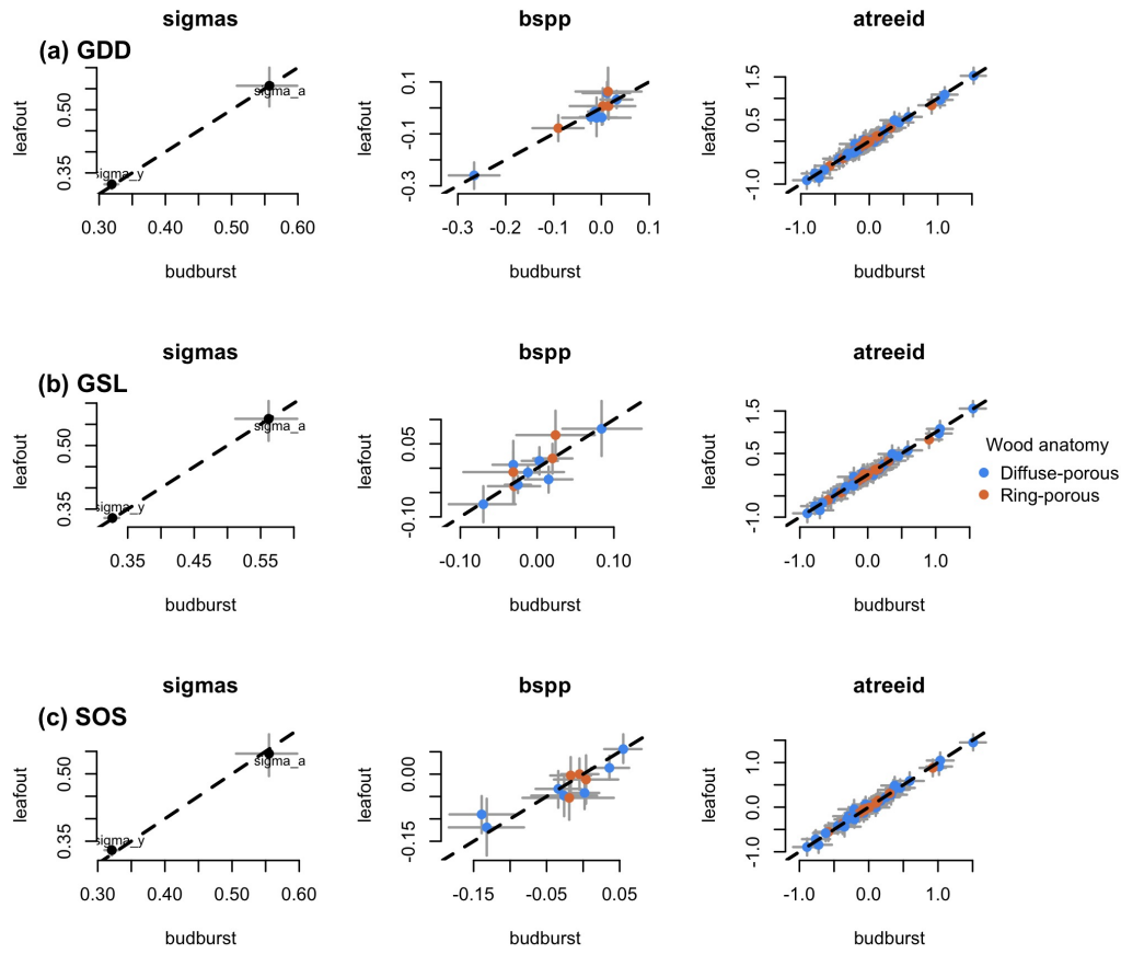
Figure S5: Parameter estimates when calculating the GDD (a), GSL (b) from leafout vs budburst, to leaf coloring. (c) shows the model estimates when taking leafout vs budburst as the SOS.
