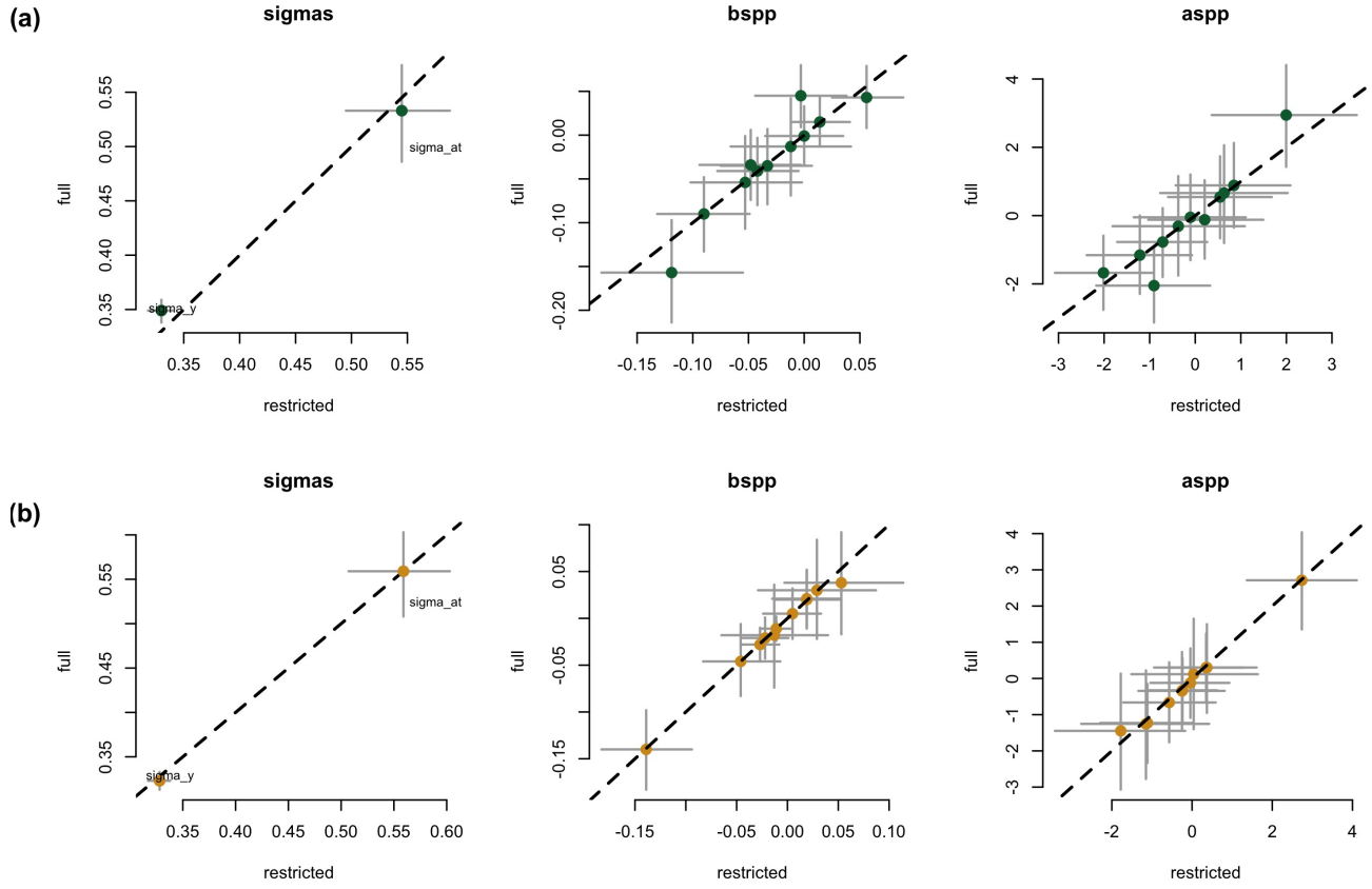
Figure S4: Full vs most restricted rows of data for the model with SOS (a) EOS (b) as the predictor for CoringTreespotter. Each panel represent the different parameters used to fit the models.
