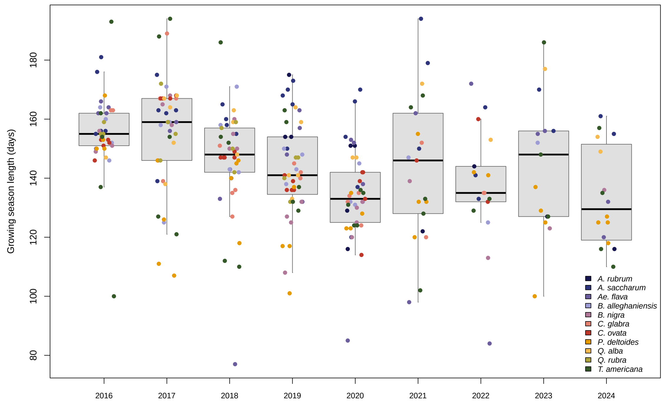
(a) Calendar season (GSL)
