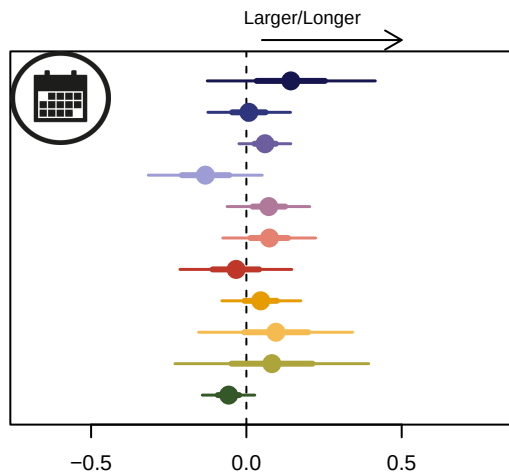
(c) Growing season length
