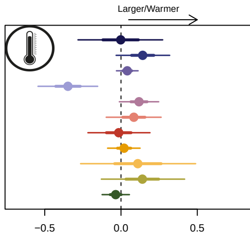
(a) Growing degree days
