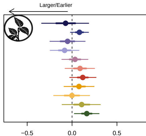
(b) Start of season
