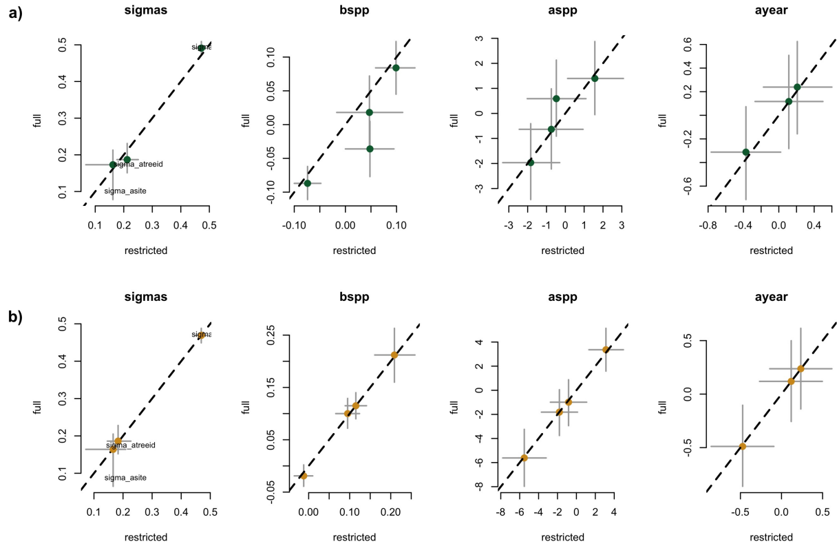
Figure S3: Full vs, most restricted rows of data for the model with start of season (SOS; a) and end of season (EOS; b) as the predictor. Each pannel represent the different parameters used to fit the models. ‘aspp’ and ‘ayear’ represent the ring width (on the log scale) deviation from the grand mean for species and year, respectively. ‘bspp’ represent the change in ring width (on the log scale) per scaled predictor for each species (see data analyses section for more details).
