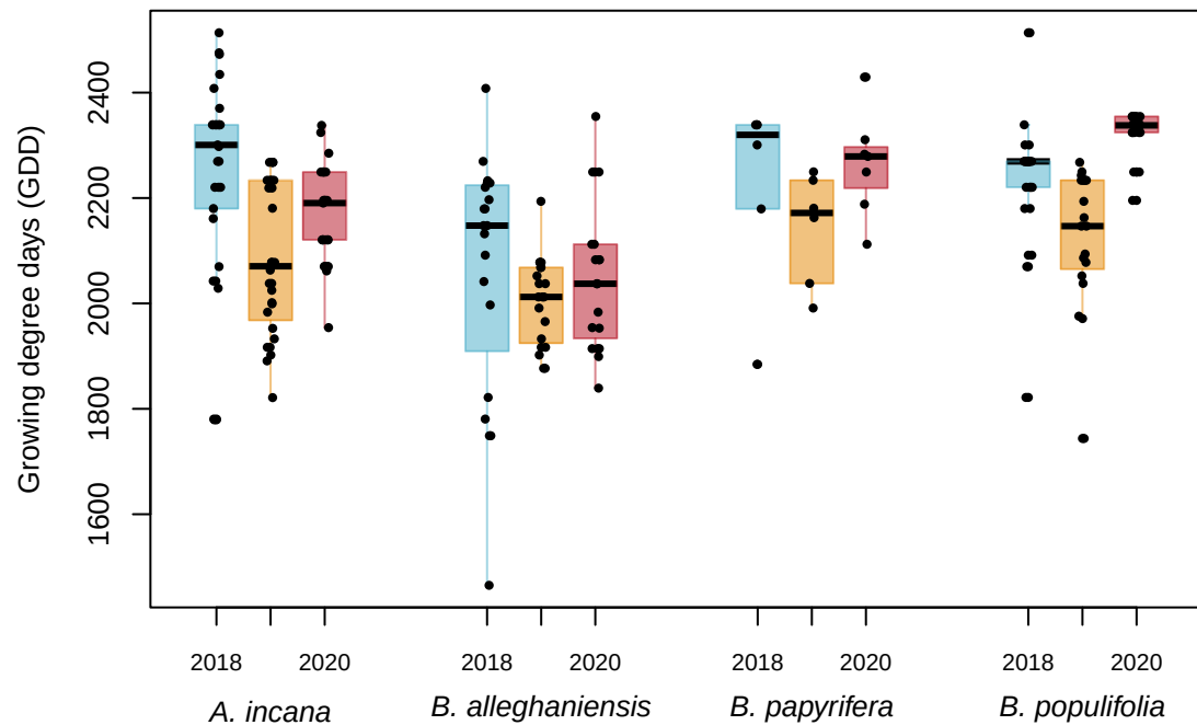
(a) Thermal season (GDD)
