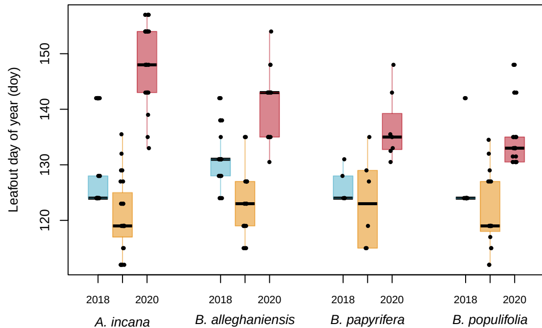
(c) Start of season (SOS)
