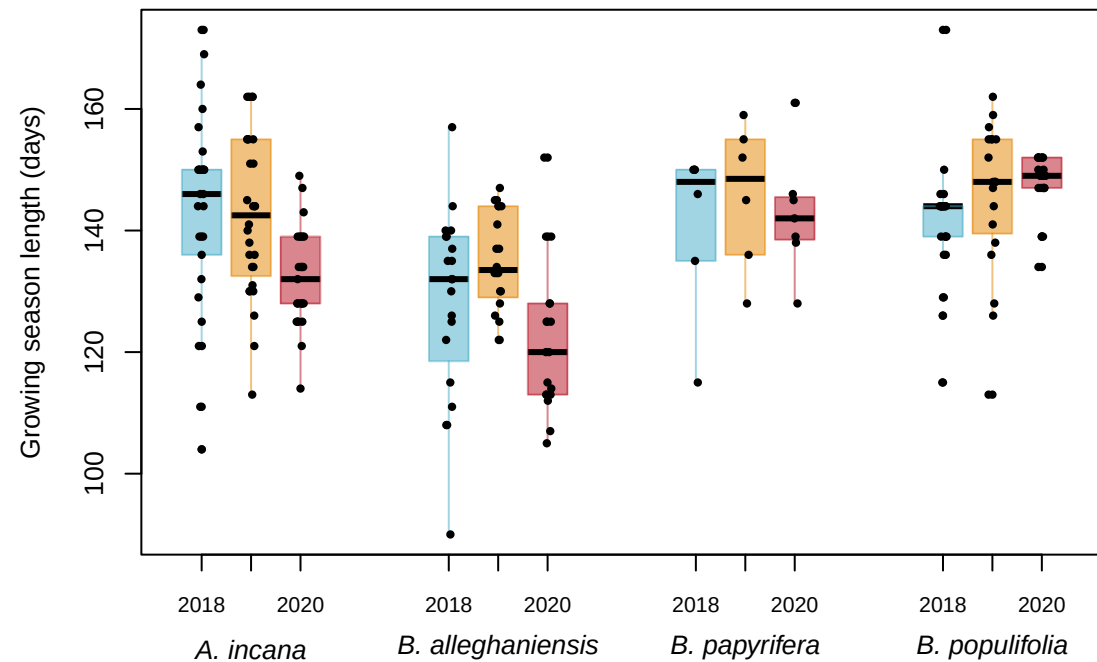
(b) Calendar season (GSL)
