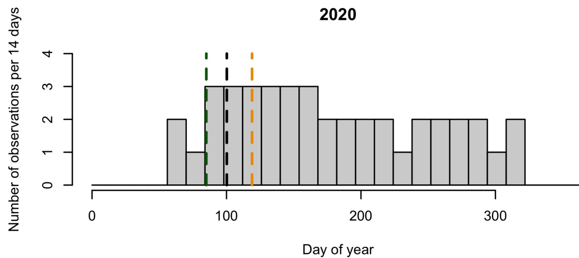
Figure 2: Phenology observations bi-weekly.
