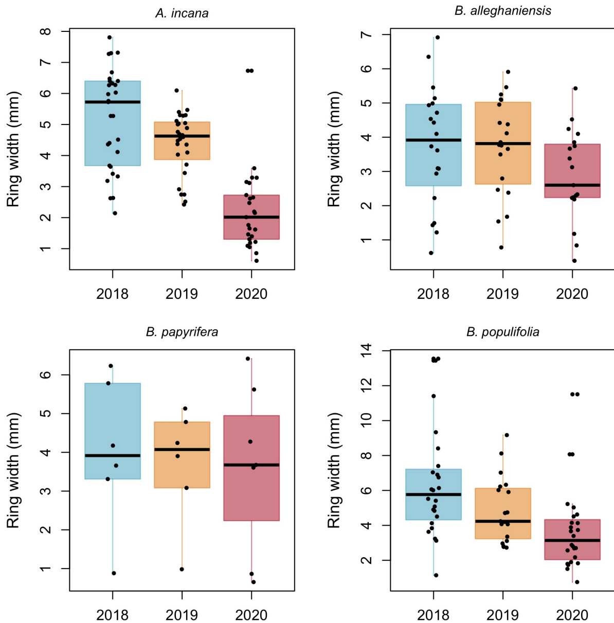
Figure S8: Boxplot representing the empirical data of our ring widths (mm) facetted by species. The dots represent the raw data, the line the mean and the box the IQR.
