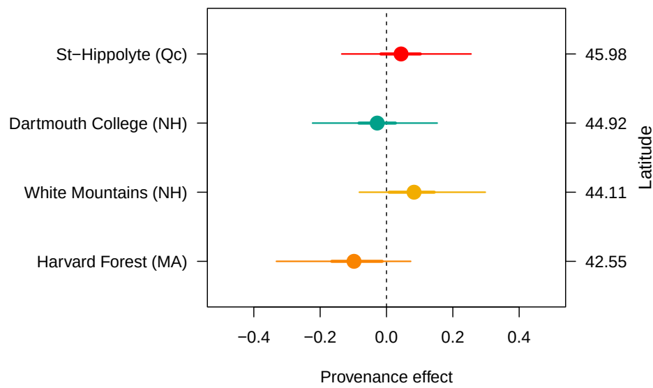
Figure 4: The effect of provenance on growth across a latitudinal gradient. We show the ring width ( \log(\text{mm}) ; see Table S2 for provenance parameter estimates) for each provenance with growing degree days as the predictor (effects were similar for the other predictors, see Tables S3, S4, S5). The dots represent the estimated mean of each provenance, with 50% and 90% uncertainty intervals (thicker and thinner lines, respectively). The provenances are color-coded from Figure 2, the map showing their locations.
