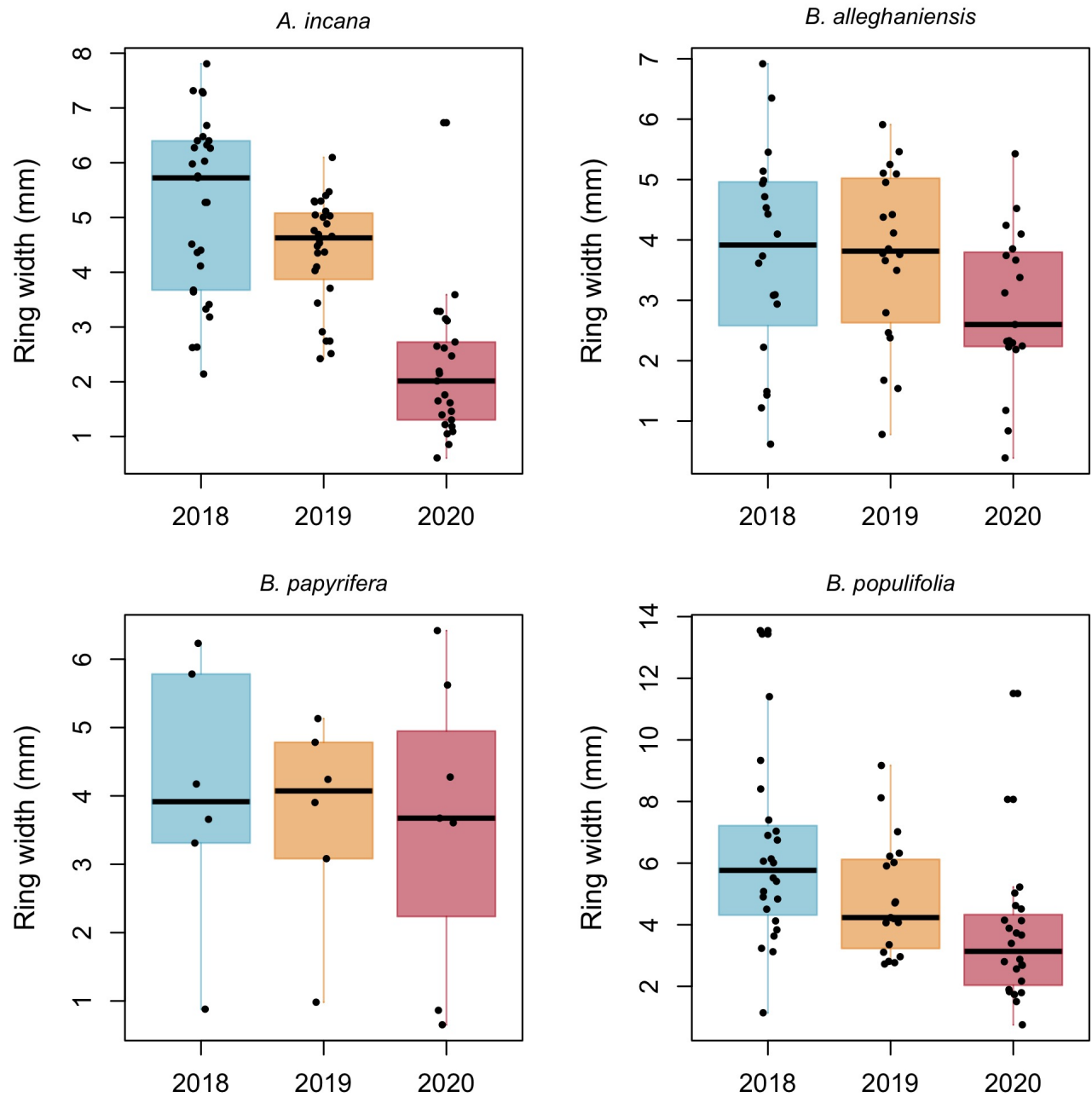
Figure S6: Empirical data. Though the trend is weak, 2020 is systematically the year with the lowest growth shown both as the mean of the model intercepts (a) and as the median of the raw data, for each species (b). The growth of 2018 and 2019 is similar.
