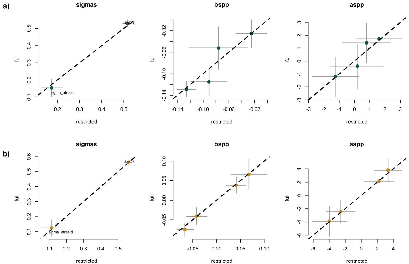
Figure S1: Full vs most restricted rows of data for the model with SOS (a) EOS (b) as the predictor for Wildchrokie. Each pannel represent the different parameters used to fit the models.
