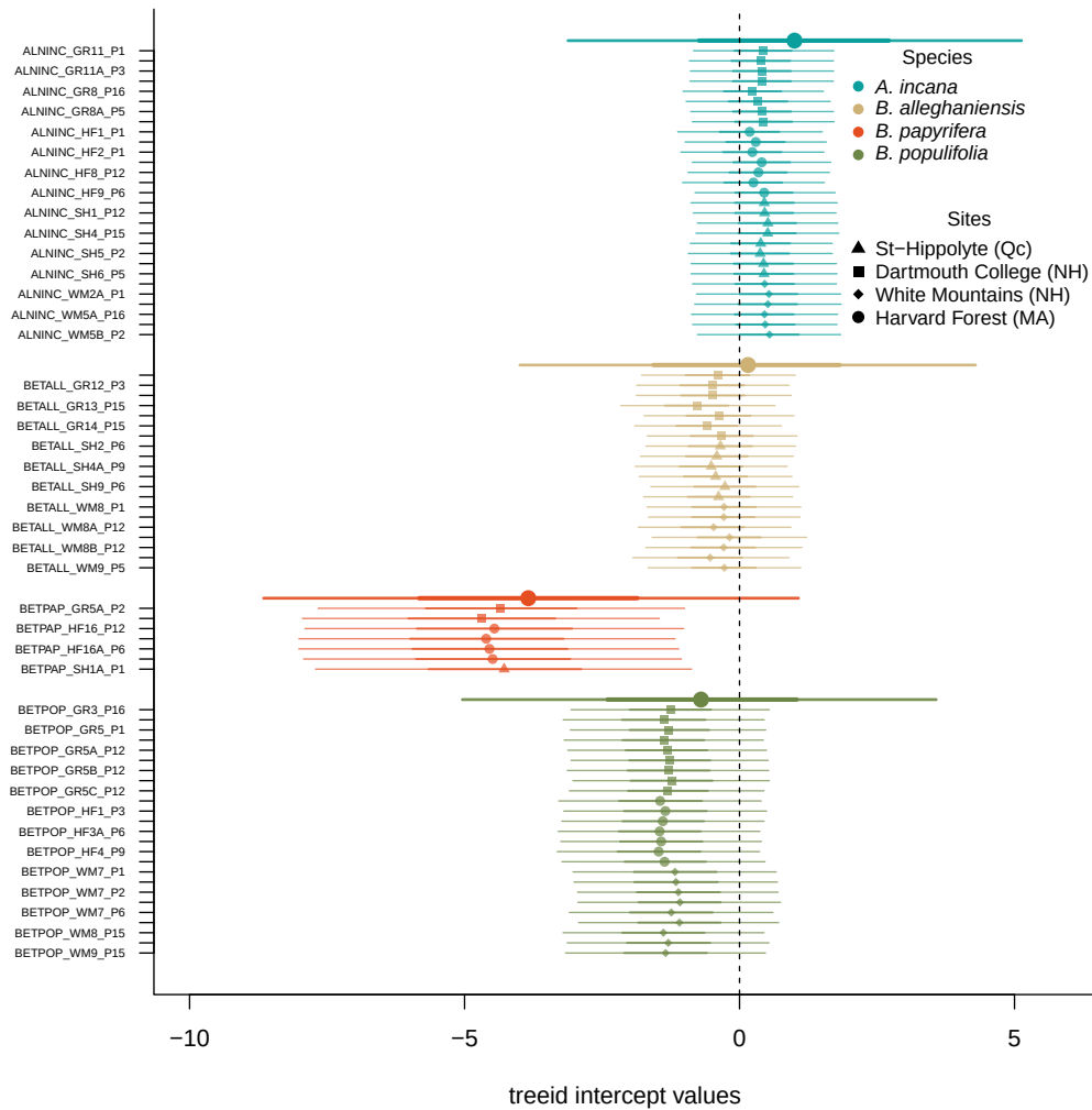
Figure S4: Intercept estimates for each group of the GDD model. The different tree id values represent the sum of the tree id, provenance, species and averaged year intercepts. The larger dots and lines represent aggregated average across these values. The dots are the mean of the posterior distribution and the thick and thin lines, the 50 and 90% UI.
