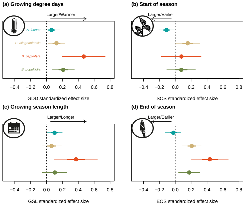
Figure S9: Effect size of each predictors across our four species. We depict ring width (on the log scale) change per scaled ( z -scored; see data analyses section for more details) predictor for each species. We report estimates as mean and 90% uncertainty intervals (in square brackets) across our four different predictors (GDD: growing degree days, GSL: growing season length, SOS: start of season and EOS: end of season).
