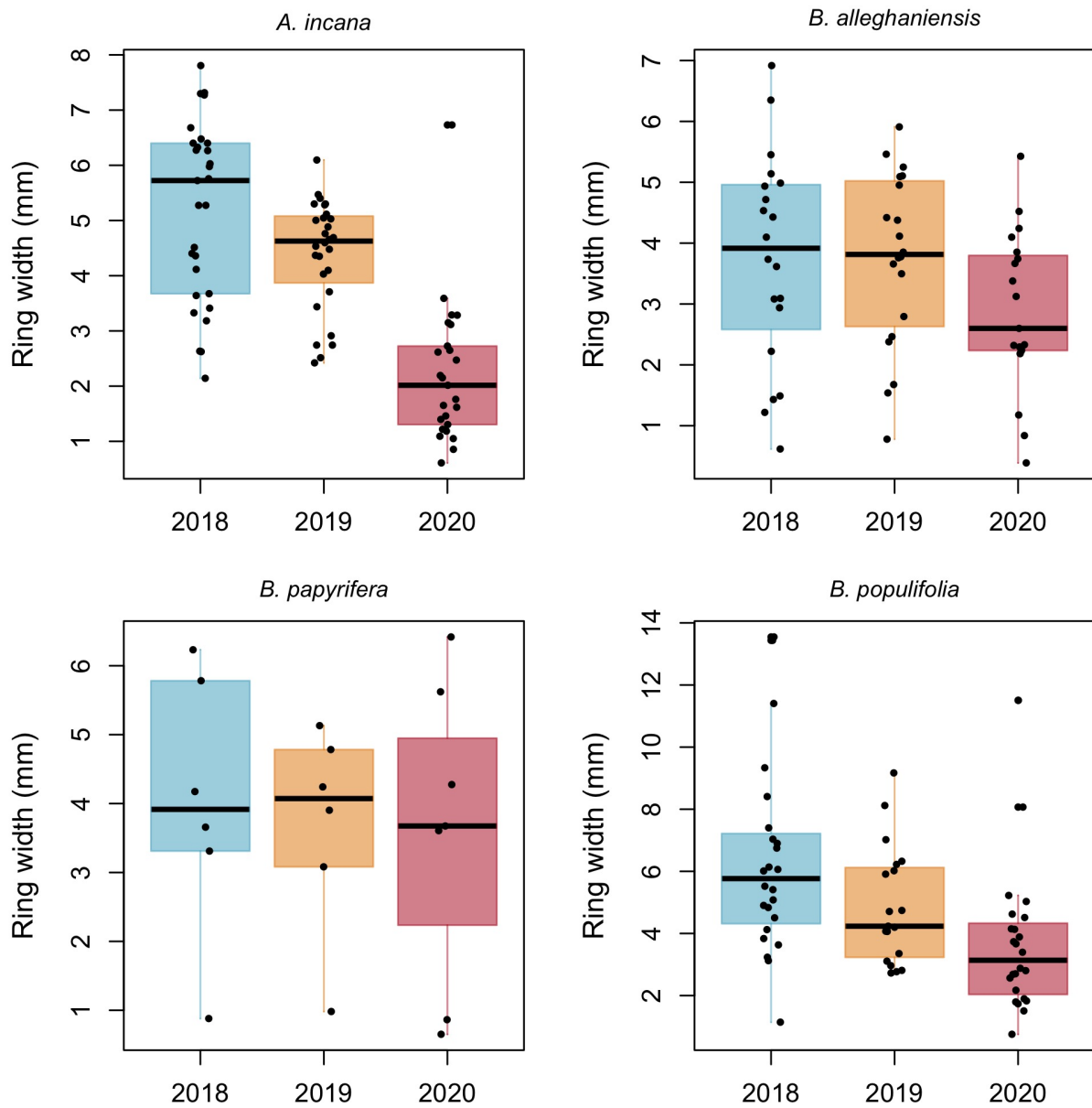
Figure S7: Boxplots representing the empirical data of our ring widths (mm) faceted by species. The dots represent the raw data, the line is the mean and the box depicts the interquartile range (IQR).
