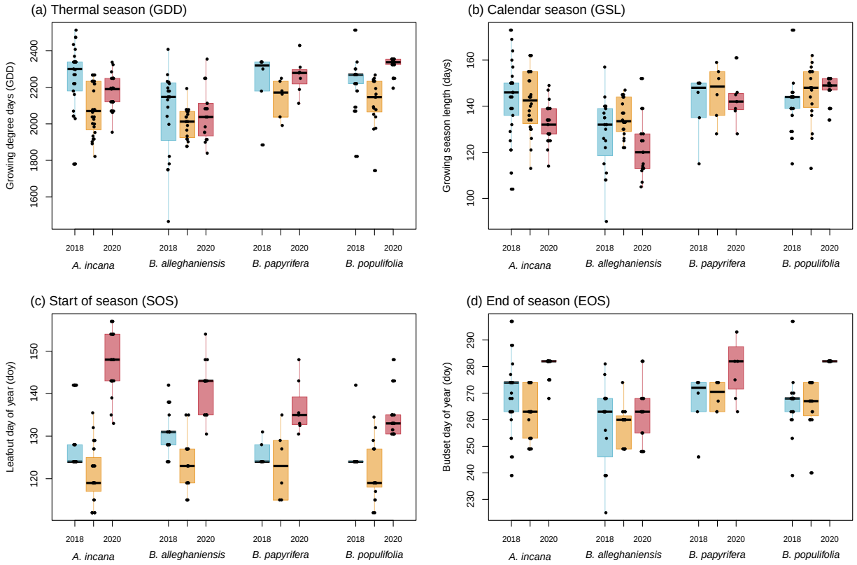
Figure S8: Boxplots representing the empirical data of all our predictors clustered by species, and for each year. The dots represent the raw data, the line is the mean and the box depicts the interquartile range (IQR).
