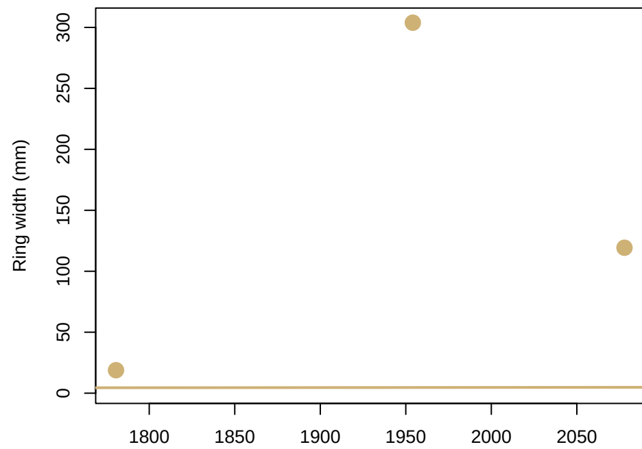
BETALL_SH9_P9
