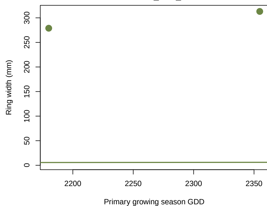
BETPOP_HF3_P1
