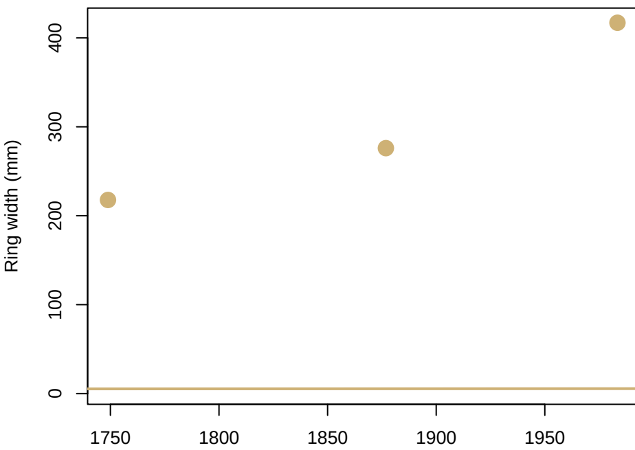
BETALL_SH9_P6
