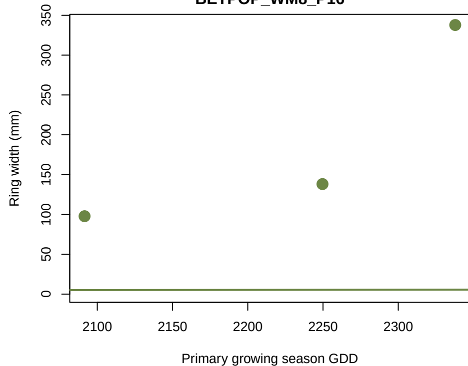
BETPOP_WM8_P16
