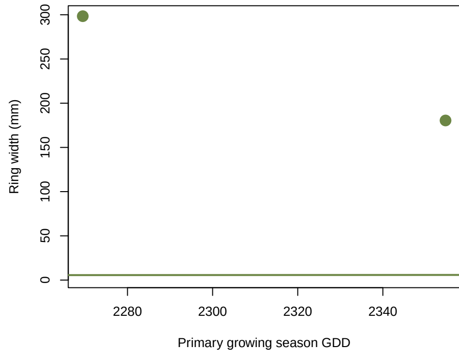
BETPOP_GR5_P6
