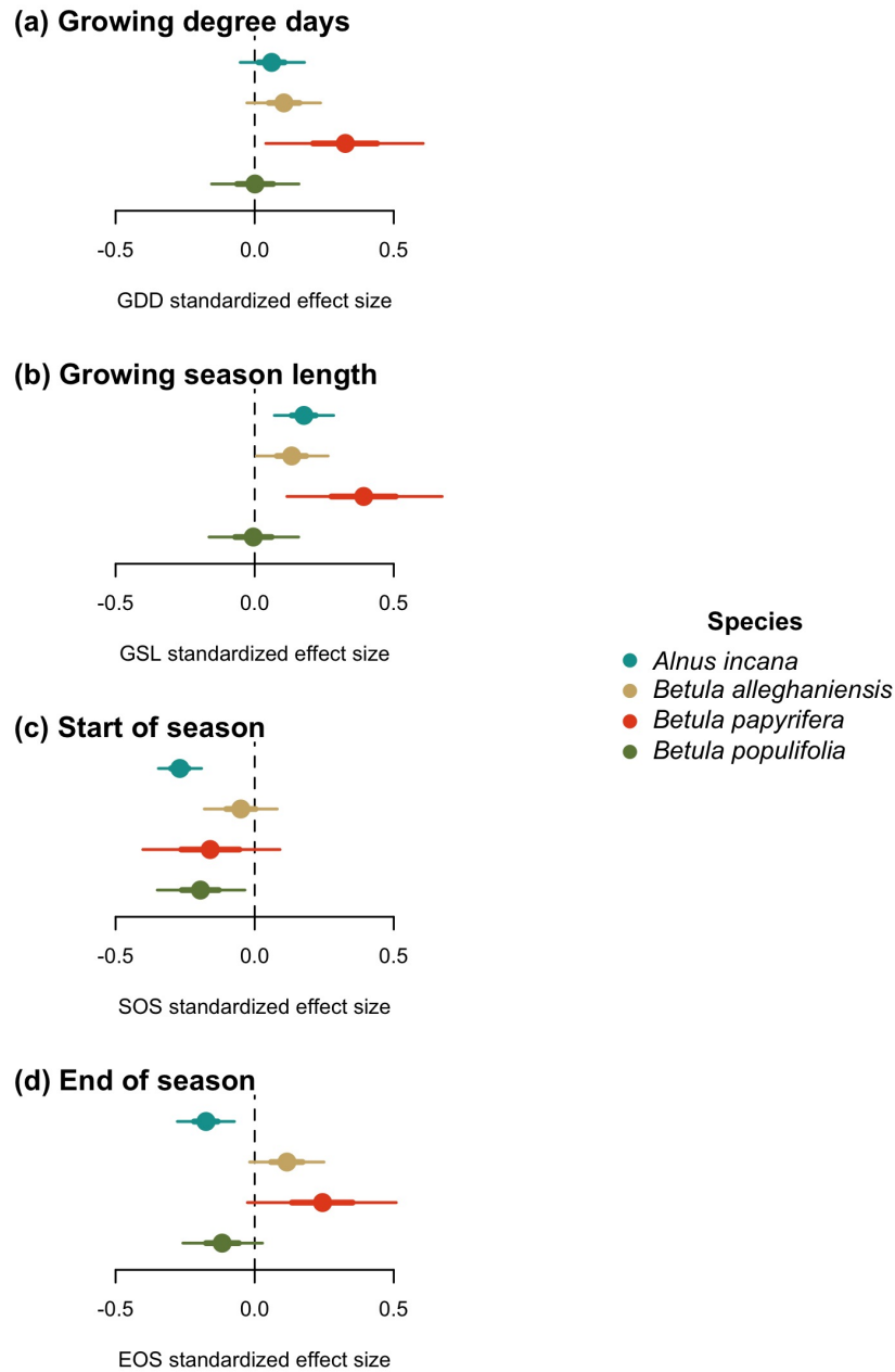
Figure S1: Standardized (z-scored) slope estimates for Wildchrokie. The dots represent the mean of the posterior distribution, the thick lines the 50% uncertainty intervals (UI) and the thinner lines, the 90% UI.
