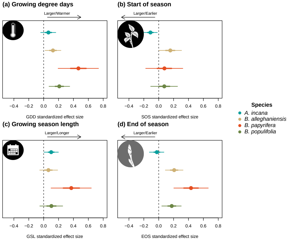
Figure S8: Standardized (z-scored) slope estimates for Wildchrokie. The dots represent the mean of the posterior distribution, the thick lines the 50% uncertainty intervals (UI) and the thinner lines, the 90% UI.
