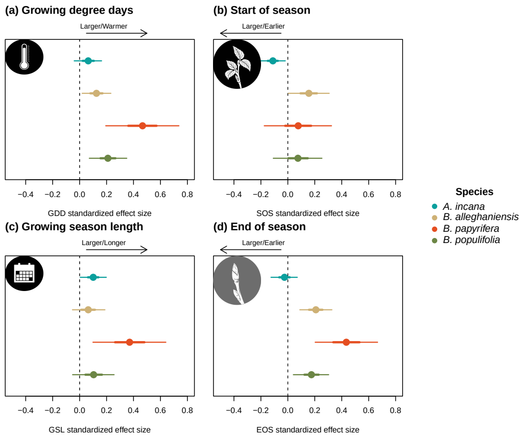
Figure S7: Standardized (z-scored) slope estimates for Wildchorkie. The dots represent the mean of the posterior distribution, the thick lines the 50% uncertainty intervals (UI) and the thinner lines, the 90% UI.
