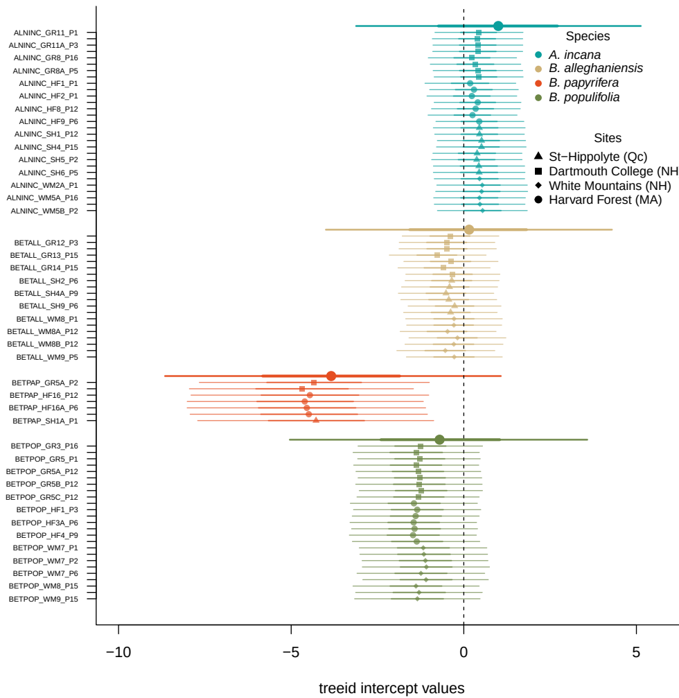
Figure S4: Intercept estimates for each group of the GDD model. The different tree id values represent the combined intercepts of tree id, provenance, species and averaged year intercepts. The bigger dots and lines represent the species intercepts which are the species level estimates averaged across all of their tree ids. The larger dots and lines represent aggregated average across these values. The dots are the mean of the posterior distribution and the thick and thin lines, the 50 and 90% UI.
