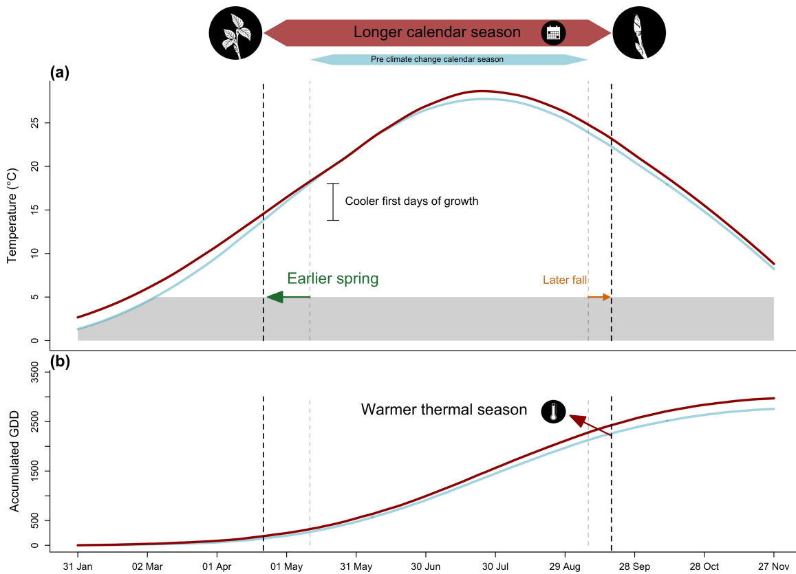
Figure 1: We show how shifting growing season length with climate change affects both the temperature experienced during the growing season (a), and how much growing degree days (GDD) they accumulate (b). We used mean daily temperature data from the Boston airport Climate station for the smoothed temperature and GDD curves. We represent the changes in temperature before (1945-1965 in blue) and after the 1980s increase in climate warming (2005-2025 in red). With climate change, spring events have advanced and fall phenology has delayed, but to much lesser extent (represented through the arrows), this lengthened the calendar growing season, but concurrently changed the temperature trees experience early in their season. As a results of increased temperature during the growing season, trees also accumulate more GDD, warming their thermal seasons.
