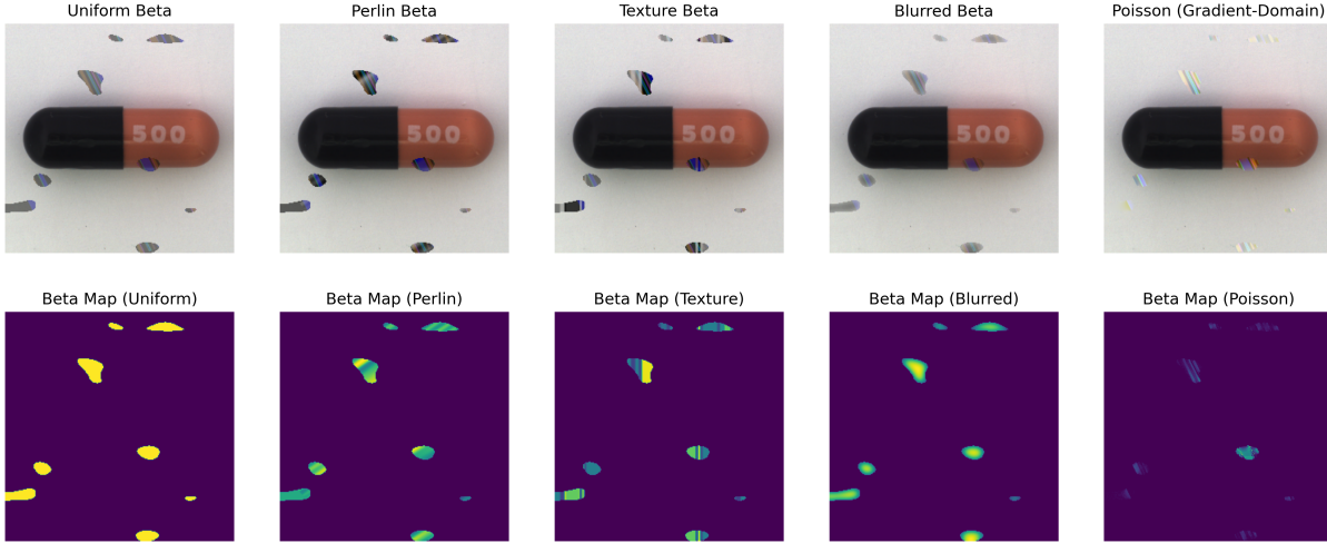
Figure 2 Different blending methods (from left to right): uniform \beta , Perlin- \beta , texture- \beta , blurred \beta , Poisson image interpolation. The top row shows an example normal image with added anomalies. The bottom row shows the strength of the contribution of the anomaly to the final image. It is clearly visible how the anomaly strength in the Poisson image interpolation is guided by the image gradients (stronger near the edge of the pill).
