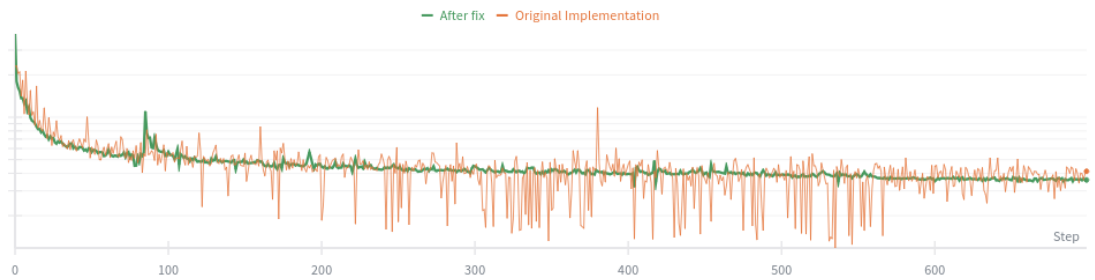
Figure 1 An example of the achieved loss smoothing by weighting the last batch of each epoch. The graph shows the SSIM loss on the training set over 700 epochs with and without correct weighting of the last incomplete batch.
