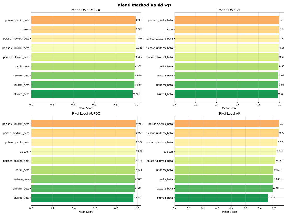
Figure 3 Combined performance comparison of blending methods and blending method combinations. The reported numbers are averages over four independent runs.
