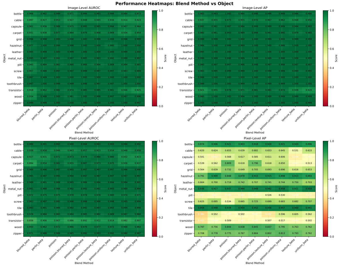
Figure 4 Detailed performance comparison of blending methods per object category. Despite performing best on average, the Poisson image interpolation (PII) blending is outperformed by other methods on some categories in terms of pixel-level AP (e.g., screw or toothbrush). The reported numbers are averages over four independent runs.
