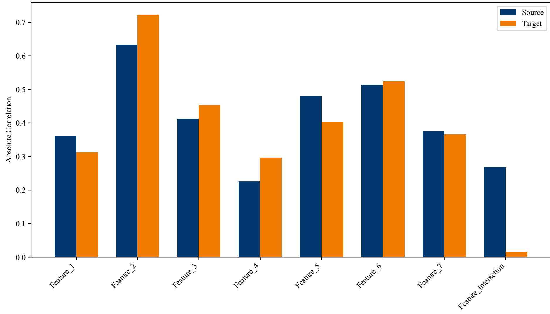
Feature Correlation with Recovery Rate (covariate)
