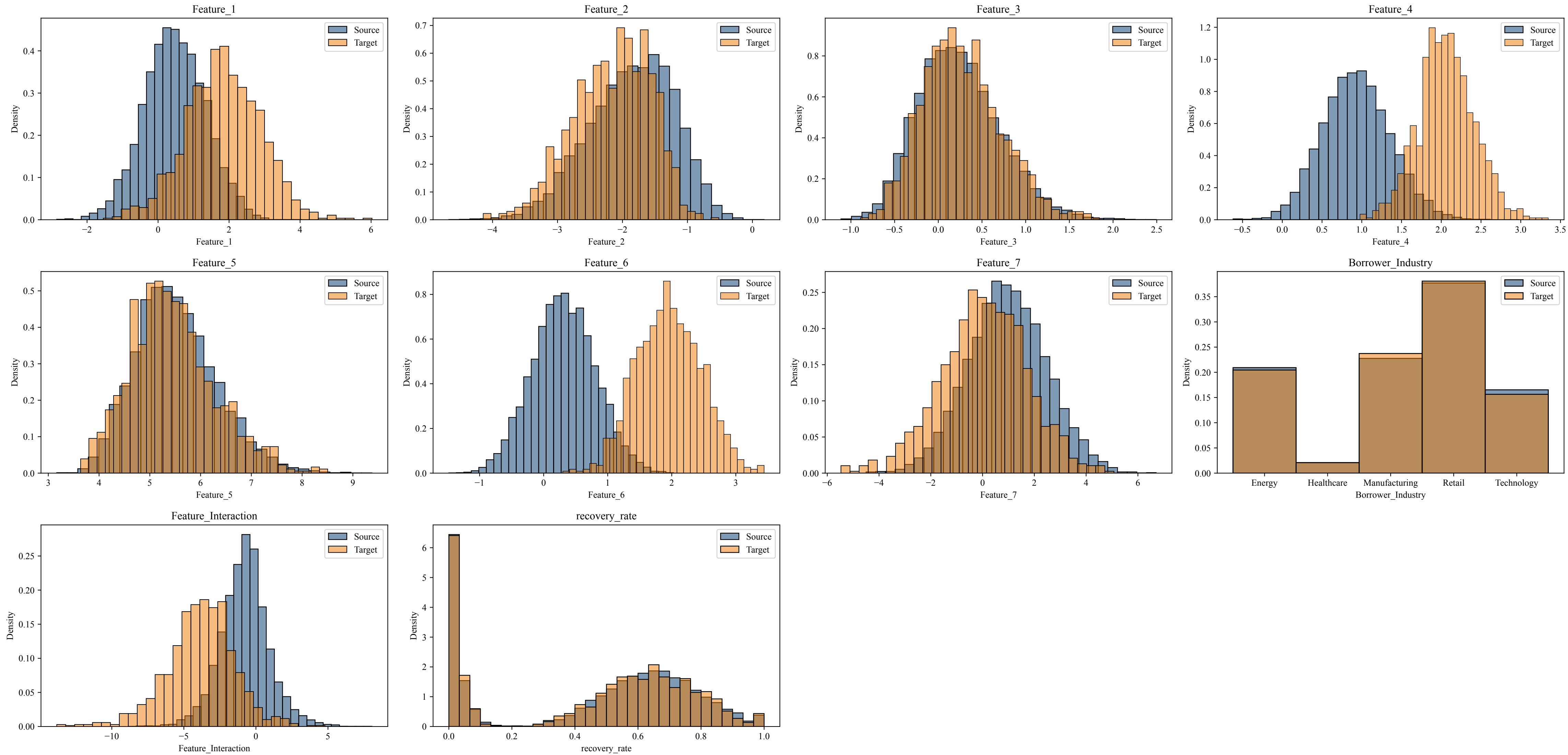
Source vs. Target Distributions (covariate)
