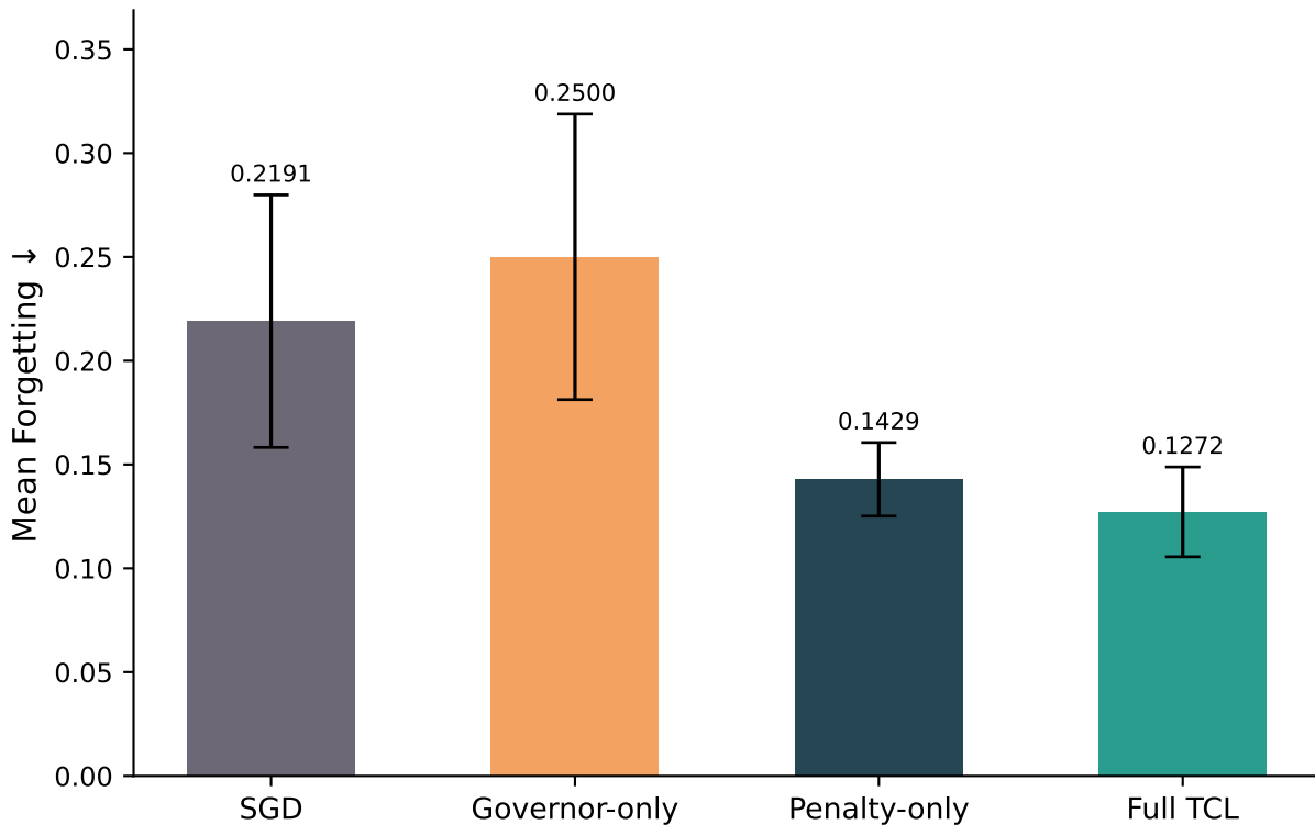
Component ablation: mean forgetting \pm std (5 seeds) Full TCL vs. isolated governor and penalty components
